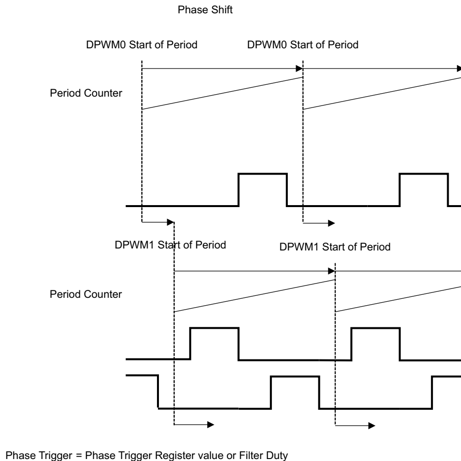
Figure 40. Phase Shifting
