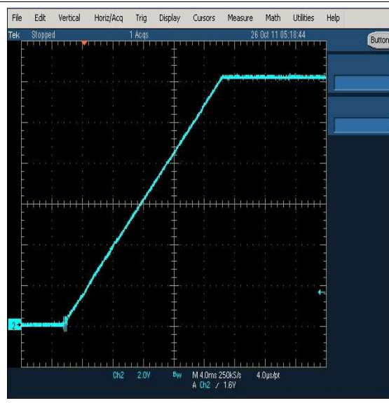
Figure 51. V_{OUT} Soft Start
