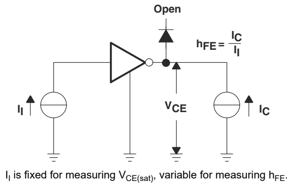
Figure 6-5. h_{FE} , V_{CE(sat)} Test Circuit
