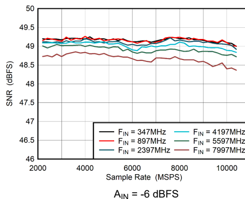
Figure 5-30. DES Mode: SNR vs Sample Rate
