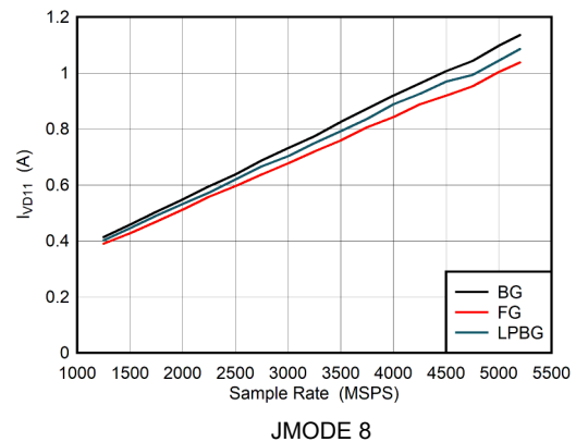
Figure 5-116. Dual Channel Mode: I_{VD11} vs Sample Rate
