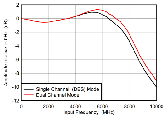
Figure 5-1. Input Amplitude vs Input Frequency
