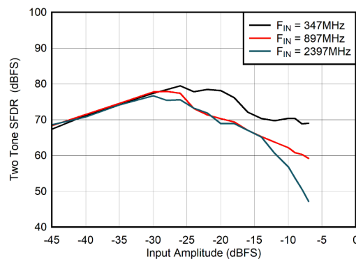
Figure 5-104. DES Mode: Two Tone SFDR vs Input Amplitude
