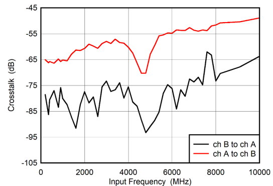
Figure 5-2. Crosstalk vs Input Frequency
