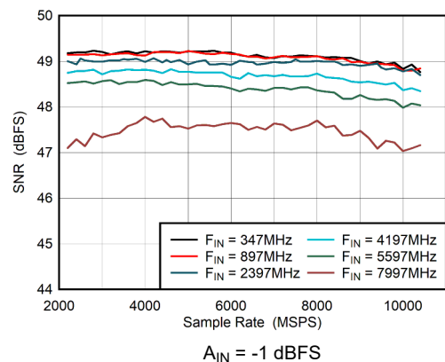
Figure 5-29. DES Mode: SNR vs Sample Rate
