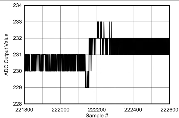
Figure 5-122. Background Calibration Core Transition (DC Signal Zoomed)
