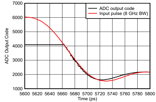
Figure 5-124. Pulse Overdrive Recovery Zoomed
