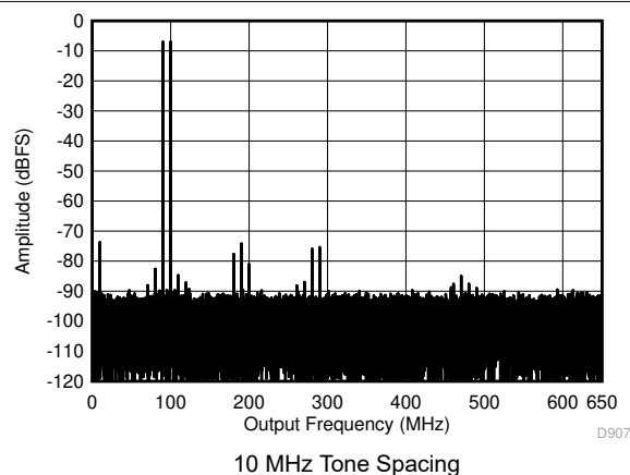
Figure 5-48. Two Tone FFT at 95.07 MHz Center
