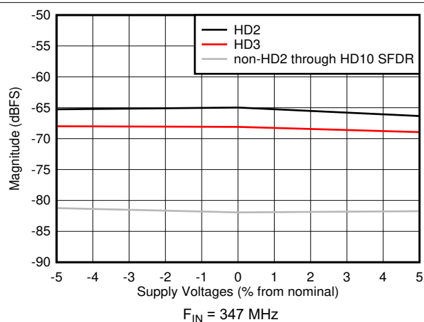
Figure 5-45. HD2, HD3 and Worst non-HD Spur vs Supply Voltage
