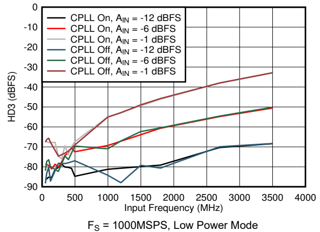
Figure 5-80. HD3 vs Input Frequency, CPLL and Input Amplitude
