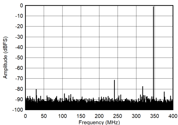
Figure 7-11. Single Tone FFT at 347MHz and -1dBFS Low Power Mode
