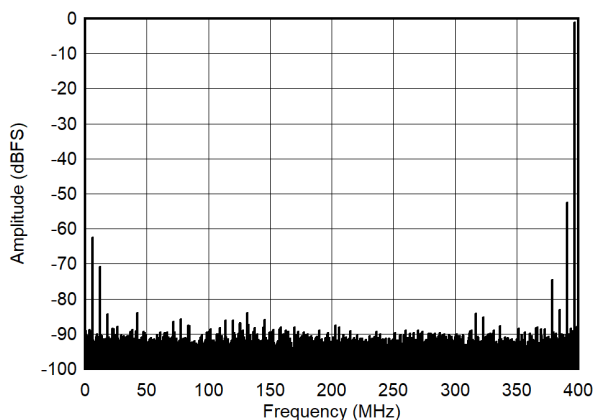
Figure 7-12. Single Tone FFT at 1197MHz and -1dBFS Low Power Mode
