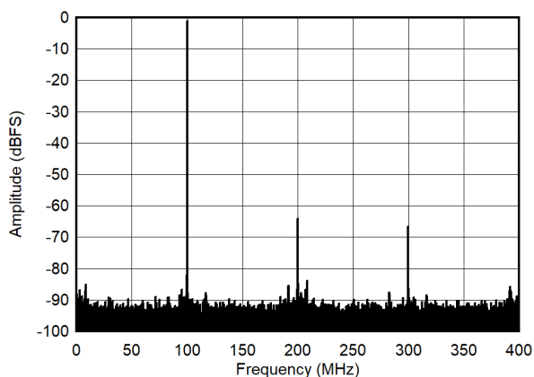
Figure 7-10. Single Tone FFT at 100MHz and -1dBFS Low Power Mode
