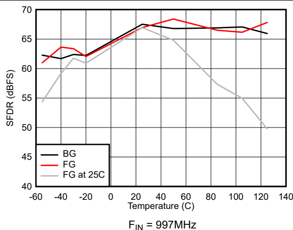
Figure 5-35. SFDR vs Temperature
