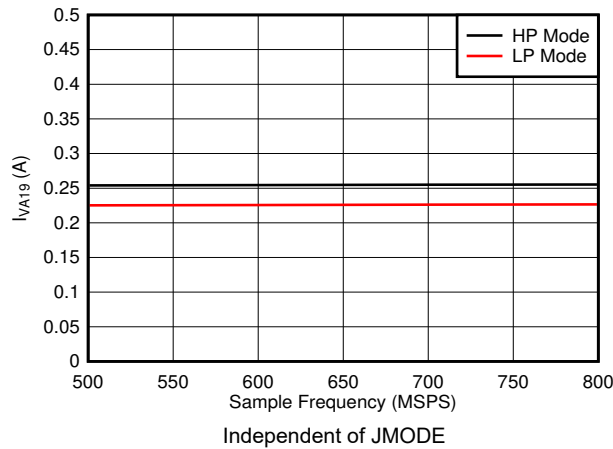
Figure 5-95. Single Channel, I_{VA19} vs F_S
