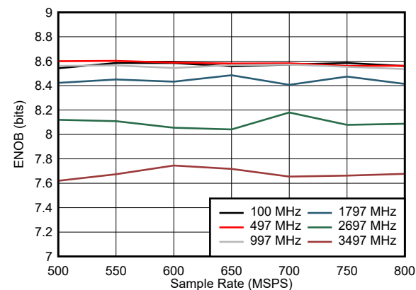
Figure 5-23. ENOB vs Sample Rate
