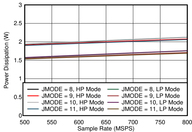
Figure 5-73. Quad Channel, Power Dissipation vs F_S for JMODES 8 - 11
