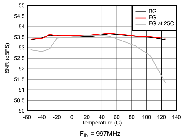
Figure 5-34. SNR vs Temperature
