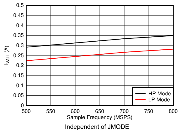
Figure 5-86. Dual Channel, I_{VA11} vs F_S
