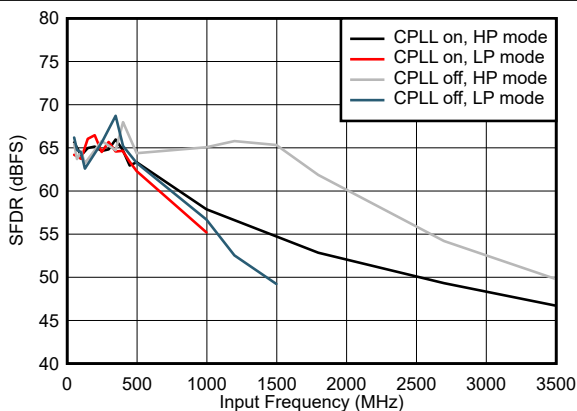
Figure 5-65. SFDR vs Input Frequency and CPLL and Power Mode
