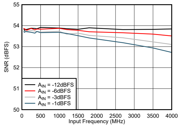
Figure 5-15. SNR vs Input Frequency
