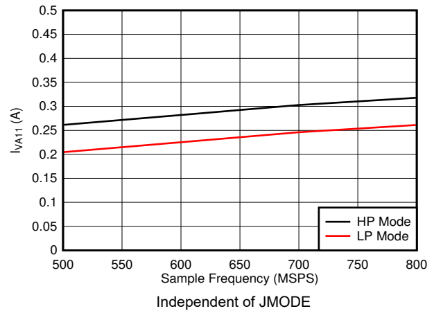
Figure 5-96. Single Channel, I_{VA11} vs F_S
