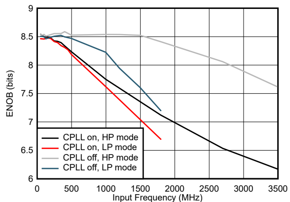
Figure 5-68. ENOB vs Input Frequency and CPLL and Power Mode
