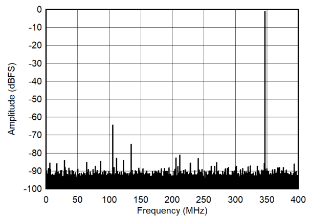
Figure 5-4. Single Tone FFT at 347 MHz and -1dBFS
