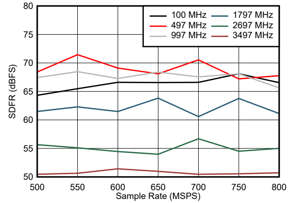
Figure 5-20. SFDR vs Sample Rate
