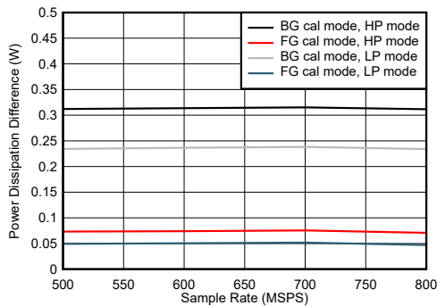
Figure 5-101. Quad Channel, Power Dissipation Change with Calibration Mode
