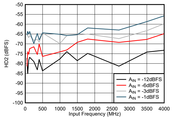
Figure 5-18. HD2 vs Input Frequency
