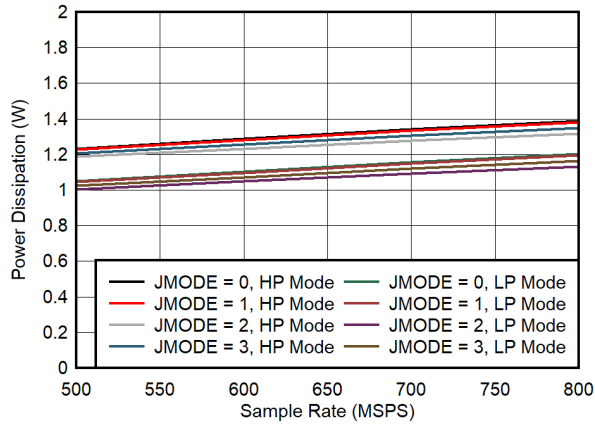
Figure 5-81. Dual Channel, Power Dissipation vs F_S for JMODES 0 - 3
