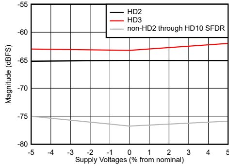
Figure 5-49. HD2, HD3 and Worst non-HD2/3 Spur vs Supply Voltage
