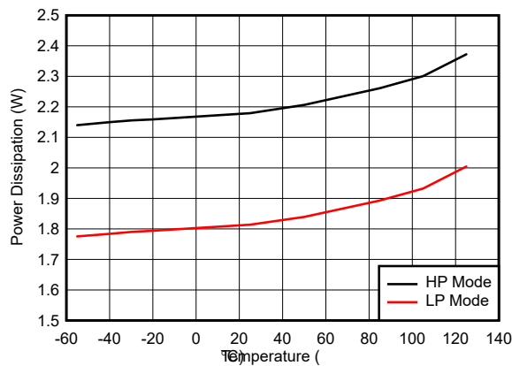
Figure 5-113. Quad Channel, Power Dissipation vs Temperature
