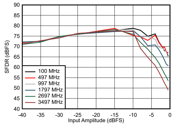
Figure 5-28. SFDR vs Input Amplitude
