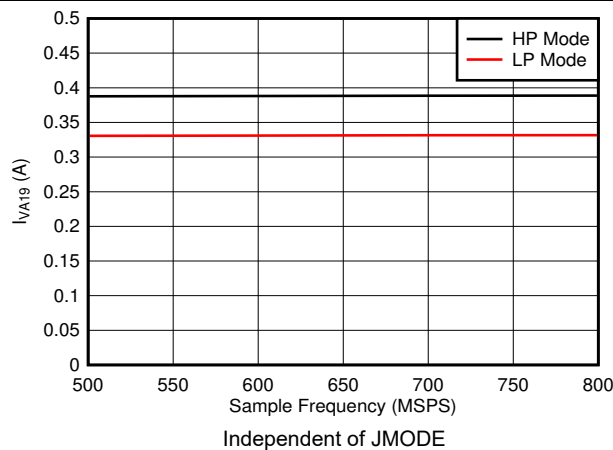
Figure 5-85. Dual Channel, I_{VA19} vs F_S
