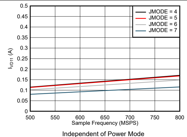
Figure 5-98. Single Channel, I_{VD11} vs F_S for JMODES 4 - 7
