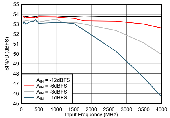
Figure 5-16. SINAD vs Input Frequency
