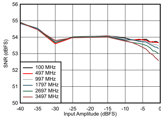
Figure 5-29. SNR vs Input Amplitude
