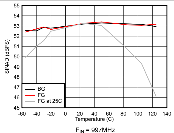
Figure 5-36. SINAD vs Temperature
