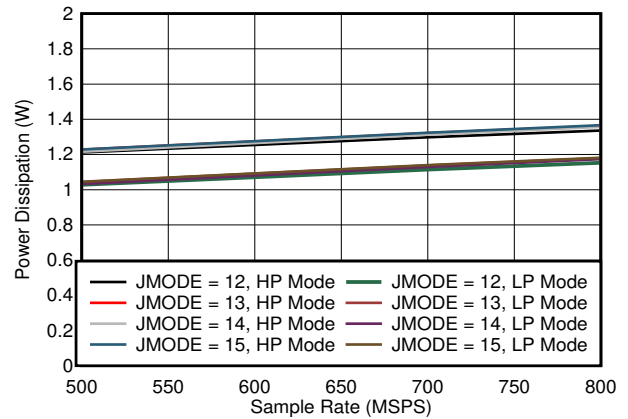
Figure 5-84. Dual Channel, Power Dissipation vs F_S for JMODES 12 - 15
