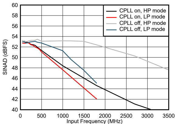
Figure 5-67. SINAD vs Input Frequency and CPLL and Power Mode
