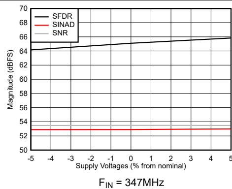
Figure 5-46. SNR, SFDR and SINAD vs Supply Voltage
