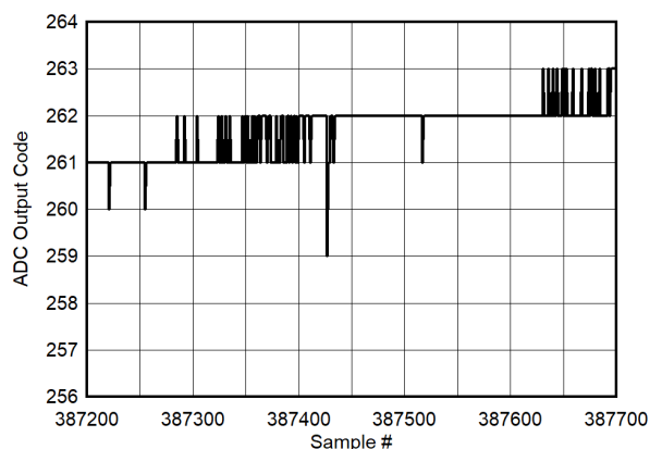
Figure 5-118. Background Core Transition (AC Signal Zoomed)
