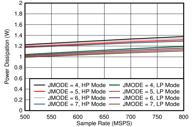
Figure 5-82. Dual Channel, Power Dissipation vs F_S for JMODES 4 - 7
