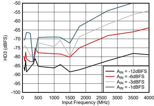
Figure 5-19. HD3 vs Input Frequency
