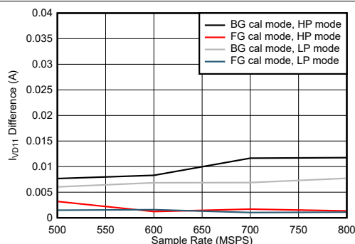
Figure 5-110. Quad Channel, I_{VD11} Change with Calibration Mode
