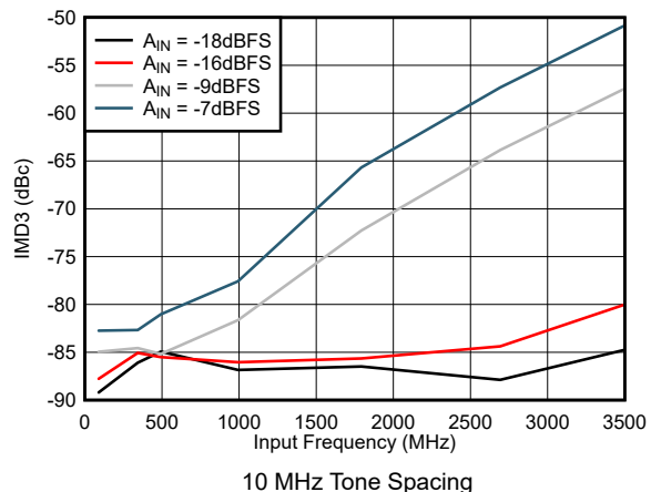
Figure 5-59. IMD3 vs Input Frequency
