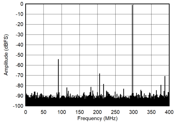
Figure 5-8. Single Tone FFT at 2697 MHz and -1dBFS
