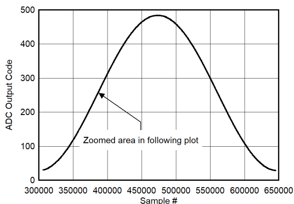
Figure 5-117. Background Core Transition (AC Signal)
