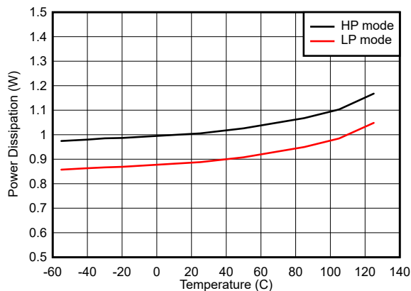
Figure 5-113. Quad Channel, Power Dissipation vs Temperature
