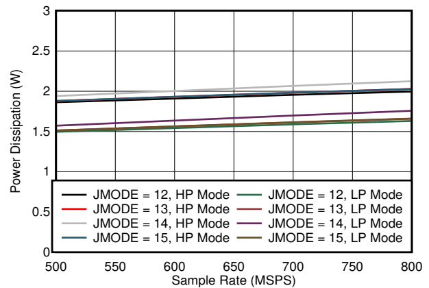
Figure 5-74. Quad Channel, Power Dissipation vs F_S for JMODES 12 - 15
