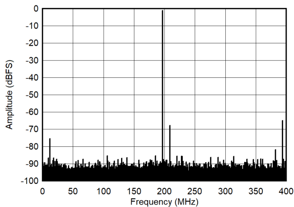
Figure 5-5. Single Tone FFT at 997 MHz and -1dBFS
