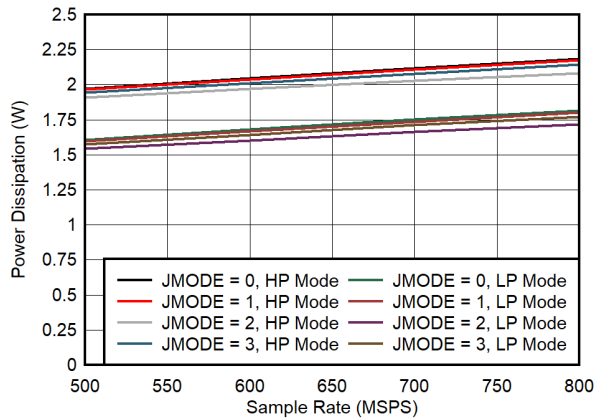
Figure 5-71. Quad Channel, Power Dissipation vs F_S for JMODES 0 - 3
