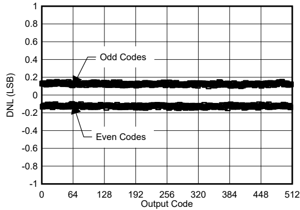
Figure 5-1. DNL vs Code
