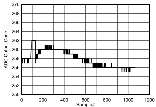
Figure 5-116. Background Core Transition (DC midscale input)
