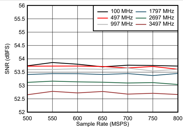
Figure 5-21. SNR vs Sample Rate
