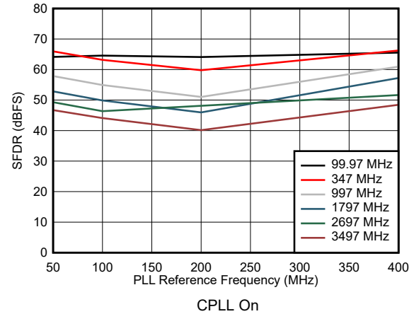
Figure 5-64. SFDR vs Reference Clock Frequency
