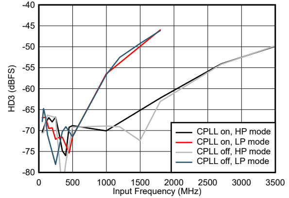
Figure 5-70. HD3 vs Input Frequency and CPLL and Power Mode
