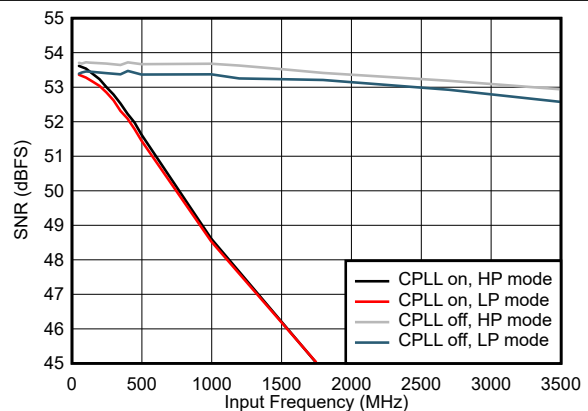
Figure 5-66. SNR vs Input Frequency and CPLL and Power Mode
