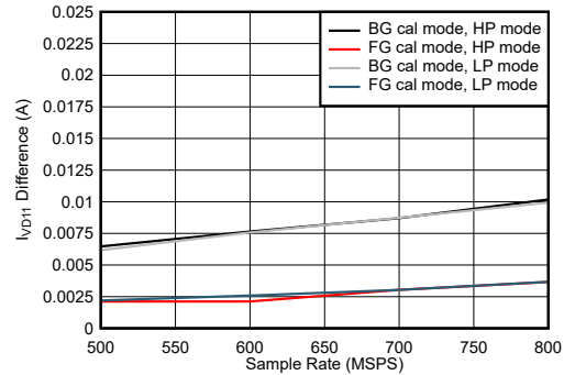
Figure 5-112. Single Channel, I_{VD11} Change with Calibration Mode
