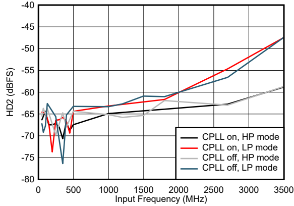
Figure 5-69. HD2 vs Input Frequency and CPLL and Power Mode
