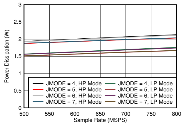
Figure 5-72. Quad Channel, Power Dissipation vs F_S for JMODES 4 - 7
