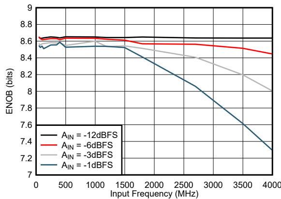
Figure 5-17. ENOB vs Input Frequency
