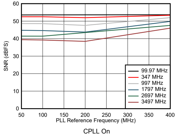
Figure 5-63. SNR vs Reference Clock Frequency
