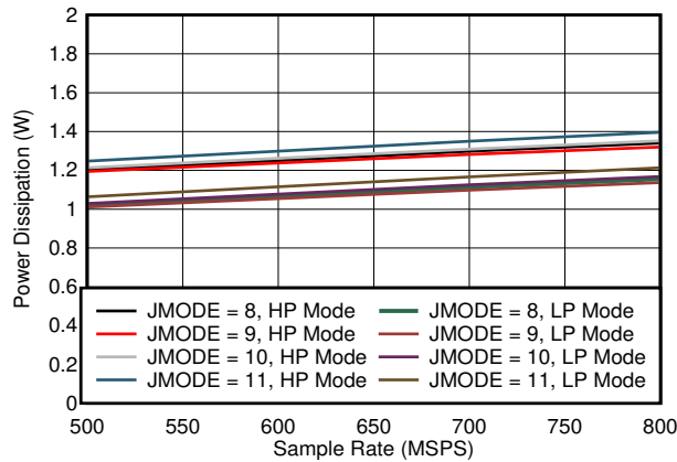
Figure 5-83. Dual Channel, Power Dissipation vs F_S for JMODES 8 - 11
