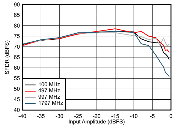
Figure 5-30. SFDR vs Input Amplitude
