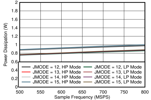
Figure 5-94. Single Channel, Power Dissipation vs F_S for JMODES 12 - 15
