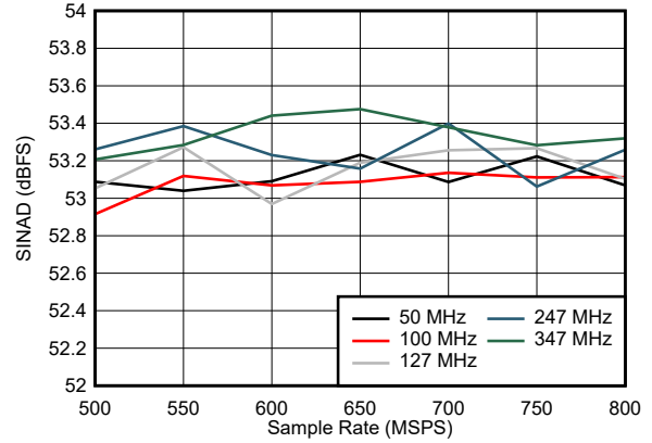
Figure 5-26. SINAD vs Sample Rate
