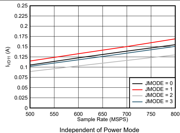
Figure 5-97. Single Channel, I_{VD11} vs F_S for JMODES 0 - 3
