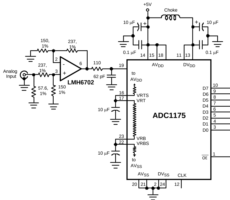
Figure 19. Simple, Low Component Count, Self-Bias Reference Application
