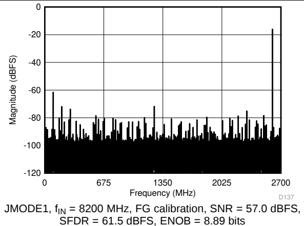
Figure 29. Single-Tone FFT at A_{\text{IN}} = -16\text{ dBFS}
