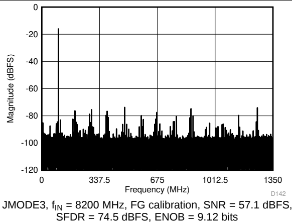
Figure 28. Single-Tone FFT at A_{\text{IN}} = -16\text{ dBFS}
