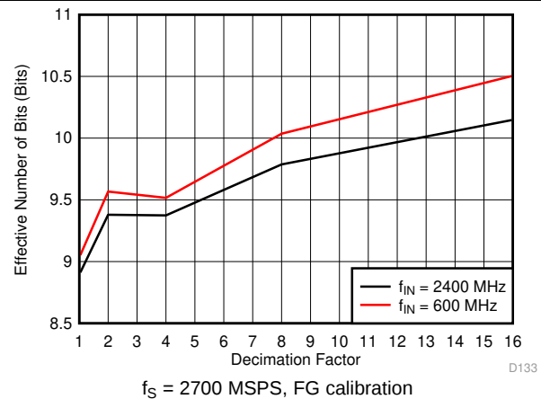
Figure 44. ENOB vs Decimation Factor
