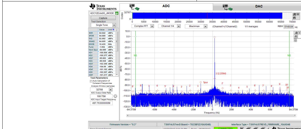
Figure 181. FFT for 497.77-MHz Input Signal, 5.4 GSPS, JMODE0
