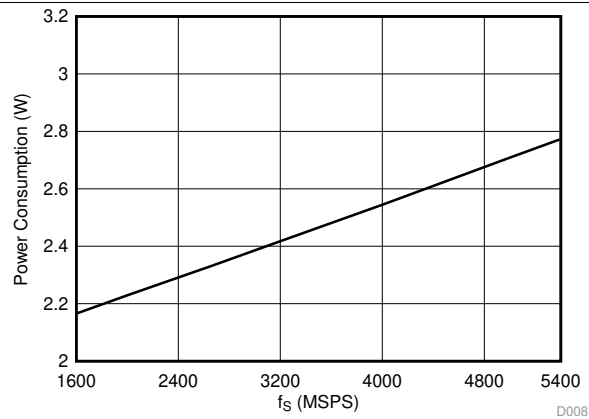
Figure 46. Power Consumption vs Sampling Rate
