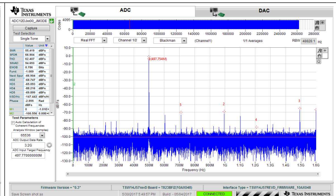
Figure 182. FFT for 497.77-MHz Input Signal, 3.2 GSPS, JMODE2
