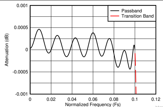
Figure 6-12. Decimate-by-4 Composite Zoomed Pass-Band Response (D4_AP87 = 0)
