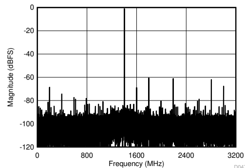
JMODE 1, FG calibration, f_s = 6400\text{MSPS} , SNR = 53.5dBFS, SFDR = 61dBFS, ENOB = 8.2 bits
