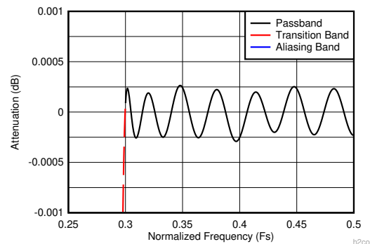
Figure 6-10. Decimate-by-2 Composite Zoomed Pass-Band Response (D2_HIGH_PASS = 1)
