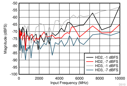
JMODE 1, f_s = 6400\text{MHz} , FG calibration
