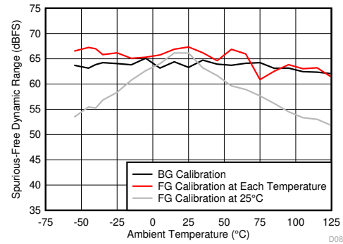
Figure 5-57. SFDR vs Temperature and Calibration Mode
