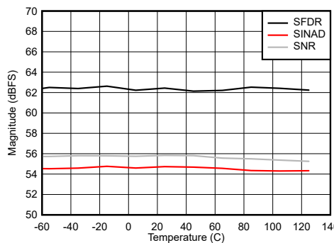
Figure 6-92. DES Mode: SNR, SINAD and SFDR vs Temperature
