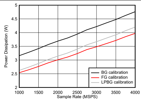
Figure 6-123. DES Mode: Power Dissipation vs Sample Rate
