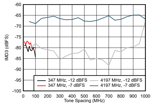
Figure 6-108. DES Mode: IMD3 vs Tone Spacing
