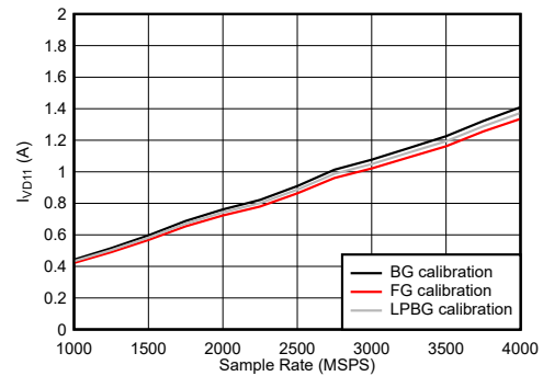
Figure 6-121. DES Mode: I_{VD11} vs Sample Rate
