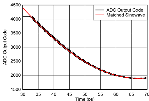
Figure 6-144. Sinewave Overdrive Recovery
