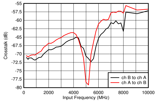
Figure 5-2. Crosstalk vs Input Frequency
