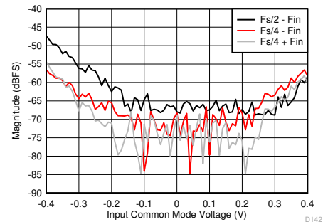
Figure 5-100. F_s/2 - F_{\text{IN}} and F_s/4 \pm F_{\text{IN}} vs Input Common Mode Voltage
