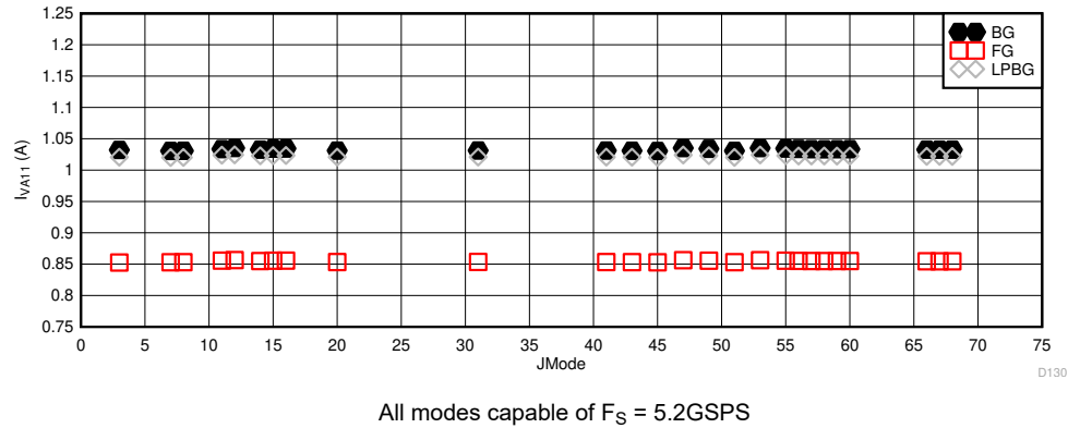
Figure 5-116. Dual Channel Mode: I_{VA11} vs \text{JMODE} at 5.2GSPS
