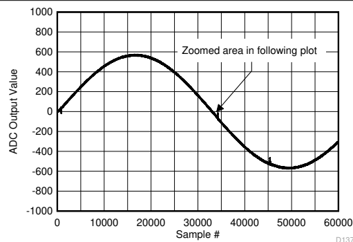
Figure 5-144. Background Calibration Core Transition (AC Signal)
