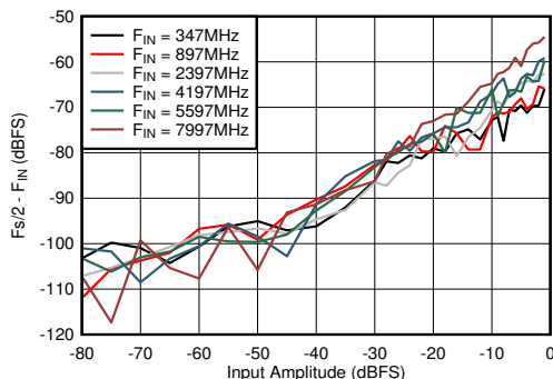
Figure 5-67. DES Mode: F_s/2 - F_{\text{IN}} vs Input Amplitude and Frequency
