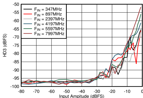
Figure 5-79. Dual Channel Mode: HD3 vs Input Amplitude and Frequency
