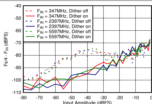
Figure 5-72. DES Mode: F_s/4 - F_{\text{IN}} vs Input Amplitude and Dither
