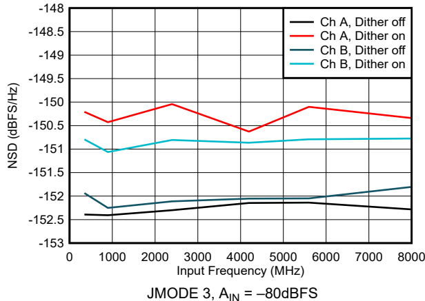
Figure 5-51. Dual Channel Mode: NSD and Input Frequency
