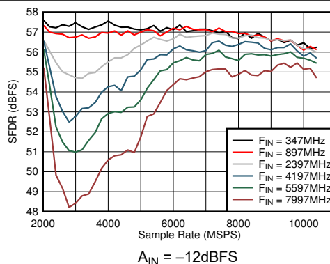
Figure 5-34. DES Mode: SFDR vs Sample Rate and Input Frequency
