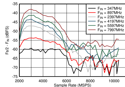
Figure 5-42. DES Mode: F_{s/2} - F_{\text{IN}} vs Sample Rate and Input Frequency
