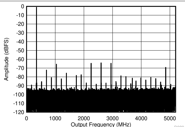
Figure 5-5. DES Mode: Single Tone FFT at 347 MHz
