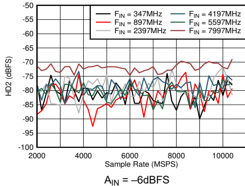
Figure 5-37. DES Mode: HD2 vs Sample Rate and Input Frequency
