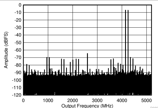
Figure 5-14. DES Mode: Two Tone FFT at 4197MHz
