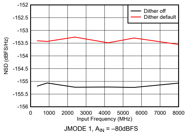
Figure 5-36. DES Mode: NSD vs Input Frequency
