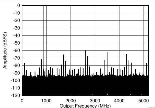
Figure 5-6. DES Mode: Single Tone FFT at 897MHz
