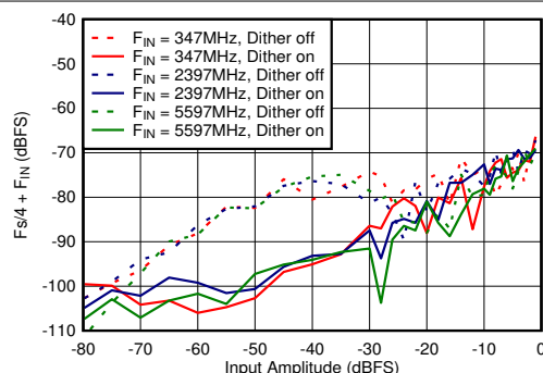
Figure 5-70. DES Mode: F_s/4 + F_{\text{IN}} vs Input Amplitude and Dither
