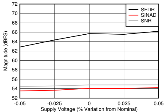
Figure 5-97. Dual Channel Mode: SNR, SINAD and SFDR vs Supply Voltage
