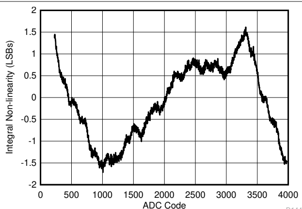
Figure 5-4. INL vs ADC Code
