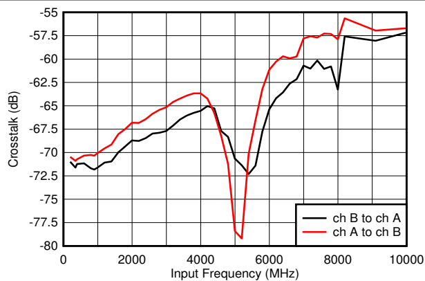
Figure 5-2. Crosstalk vs Input Frequency
