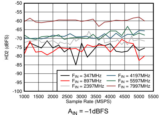
Figure 5-52. Dual Channel Mode: HD2 vs Sample Rate and Input Frequency
