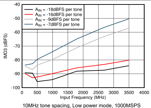
Figure 6-76. IMD3 vs F_{IN}
