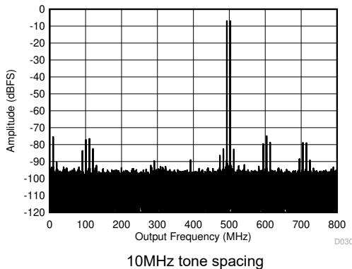
Figure 6-69. Two Tone FFT at 498MHz
