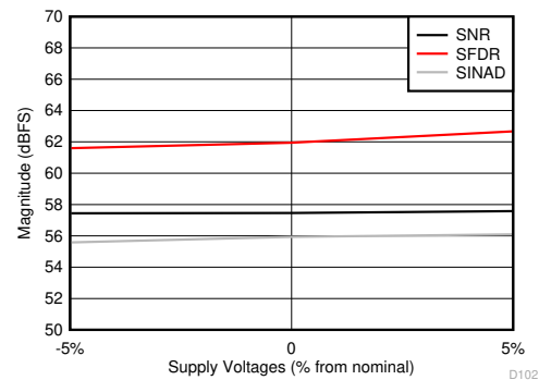
All supplies changed together, low power mode, F_S = 1000 MSPS Figure 6-62. SNR, SFDR and SINAD vs Supply Voltages
