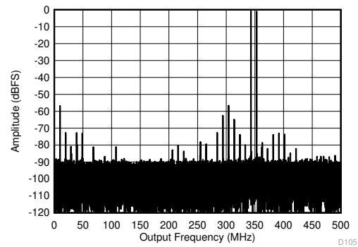
Figure 6-72. Two Tone FFT at 348 MHz
