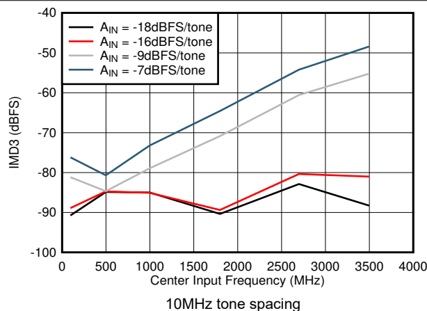
Figure 6-75. IMD3 vs F_{IN}
