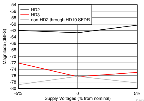
All supplies changed together, low power mode, F_S = 1000 MSPS Figure 6-63. HD2, HD3 and Worst non-HD Spur vs Supply Voltage
