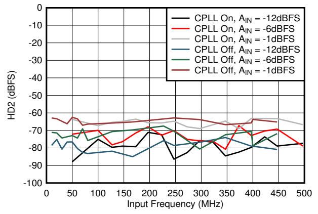
Figure 6-58. HD2 vs A_{IN} and C-PLL
