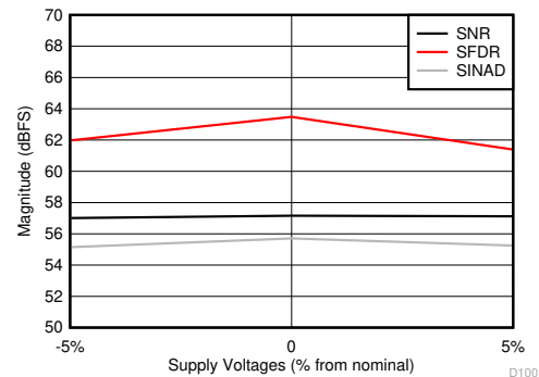
All supplies changed together, high power mode Figure 6-60. SNR, SFDR and SINAD vs Supply Voltage
