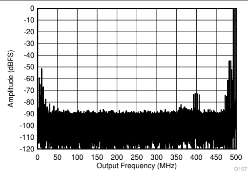
Figure 6-74. Two Tone FFT at 3498 MHz
