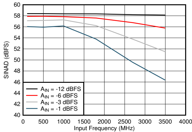
Figure 6-19. SINAD vs Input Frequency
