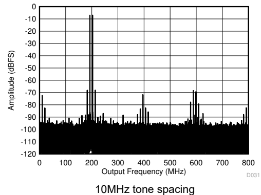
Figure 6-70. Two Tone FFT at 1798MHz
