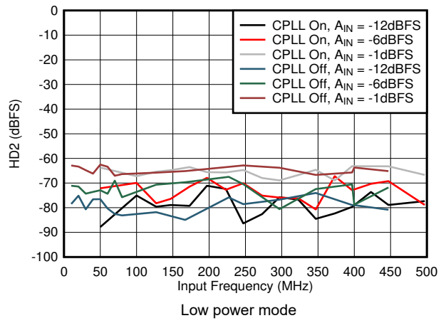
Figure 7-58. HD2 vs A_{IN} and C-PLL
