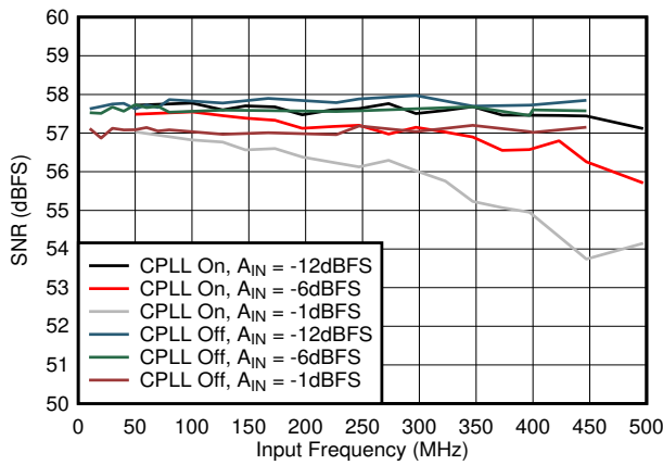
Figure 7-55. SNR vs A_{IN} and C-PLL
