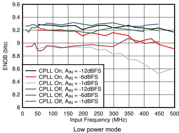
Figure 7-57. ENOB vs A_{IN} and C-PLL
