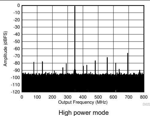
Figure 5-4. Single Tone FFT at 347 MHz and -1 dBFS
