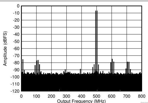
10MHz tone spacing Figure 5-69. Two Tone FFT at 498MHz
