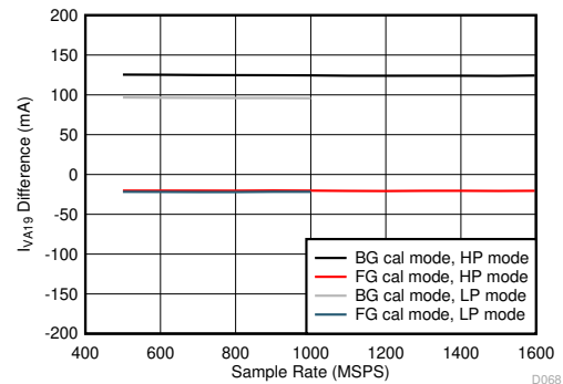
Figure 5-112. Quad Channel, I_{VA19} Change with Calibration Mode
