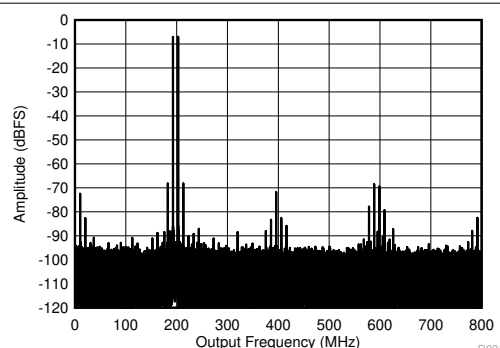
10MHz tone spacing Figure 5-70. Two Tone FFT at 1798MHz
