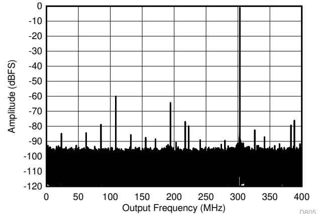
Figure 5-8. Single Tone FFT at 2097 MHz and -1dBFS
