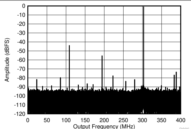
Figure 5-12. Single Tone FFT at 2097 MHz and -1dBFS
