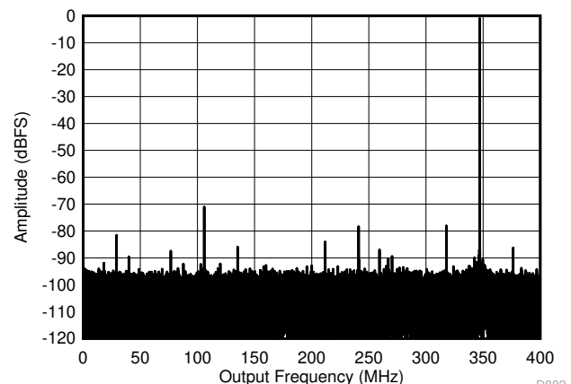
Figure 5-10. Single Tone FFT at 347 MHz and -1dBFS
