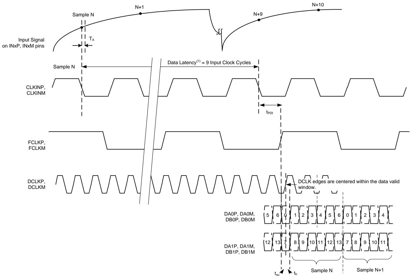
Figure 42. Latency Diagram
