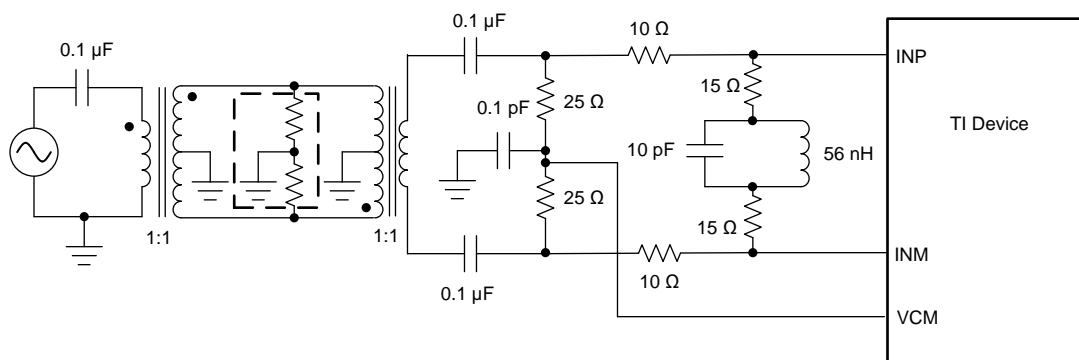
Figure 87. Driving Circuit for Mid-Range Input Frequencies ( 100 \text{ MHz} < f_{\text{IN}} < 230 \text{ MHz} )
