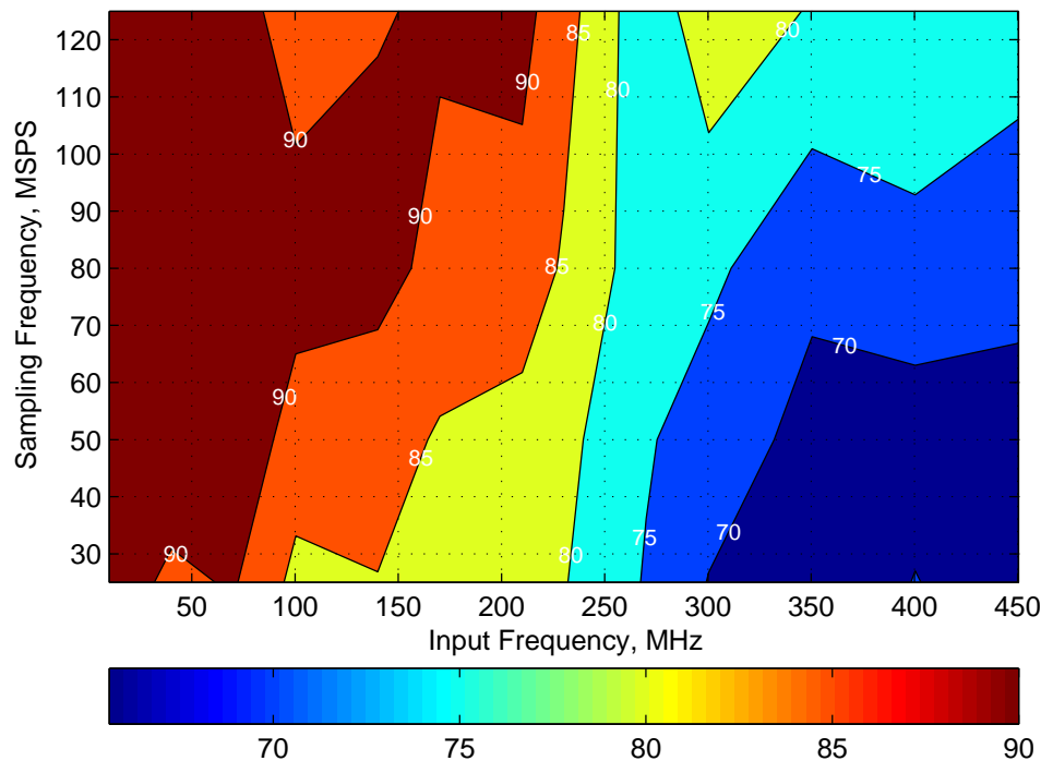
Figure 37. Spurious-Free Dynamic Range (SFDR)
