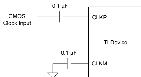
Figure 47. Single-Ended Clock Driving Circuit
