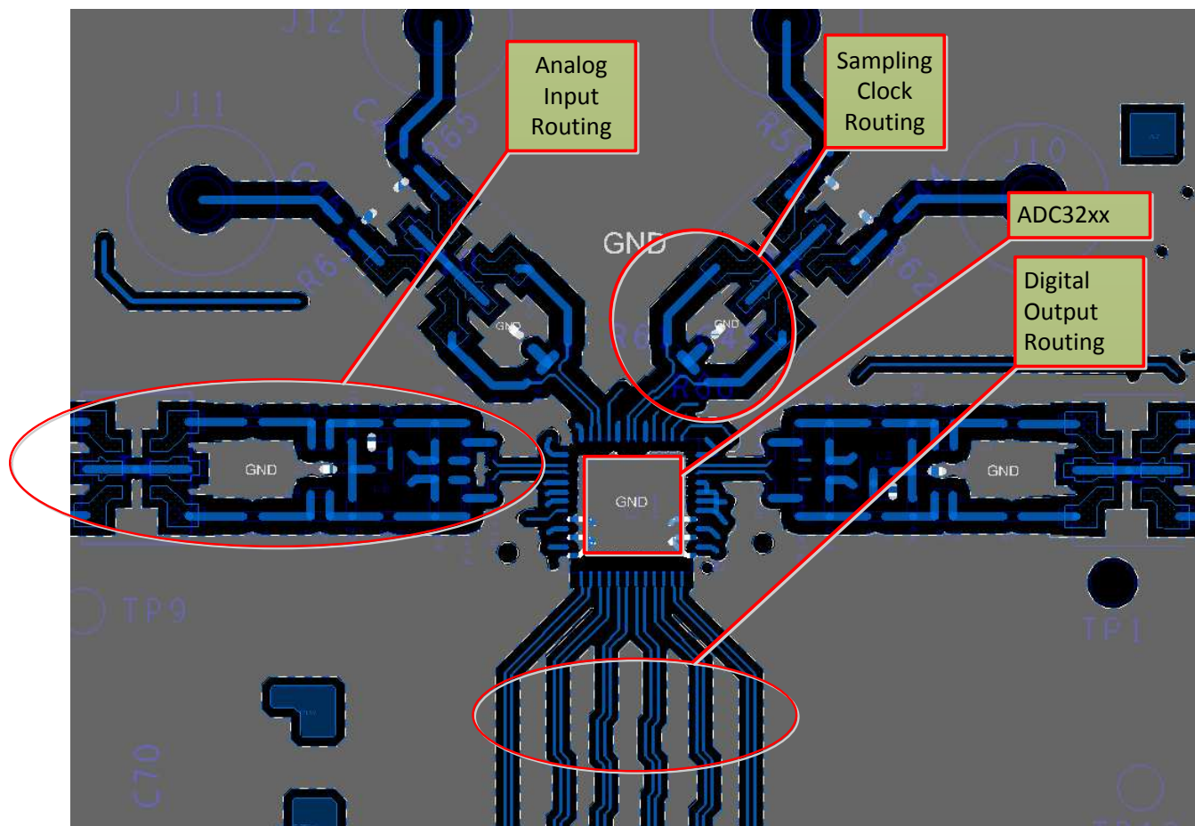
Figure 91. Typical Layout of the ADC3244E Board
