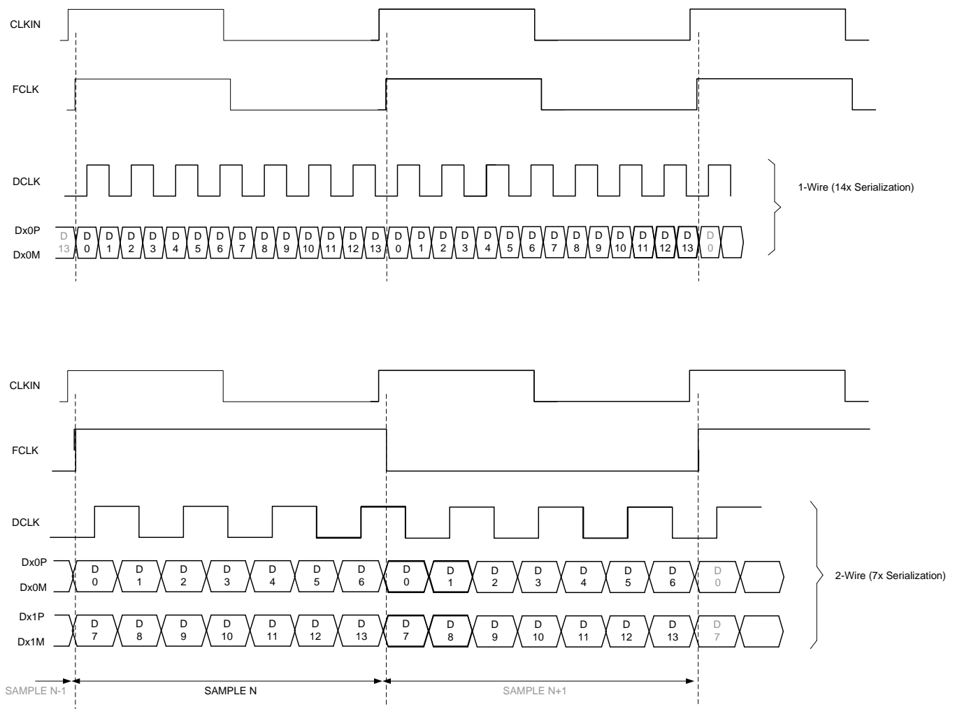
Figure 40. Output Timing Diagram
