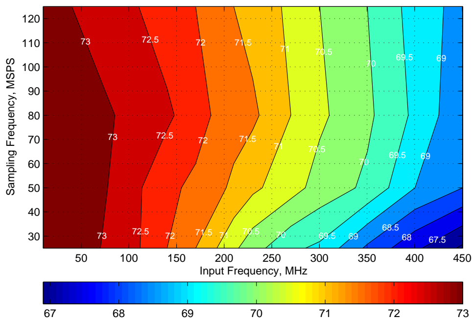
Figure 38. Signal-to-Noise Ratio (SNR)
