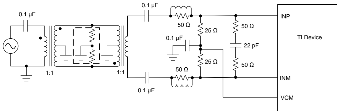
Figure 85. Driving Circuit for Low Input Frequencies
