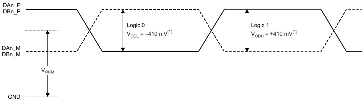
Figure 39. Serial LVDS Output Voltage Levels
