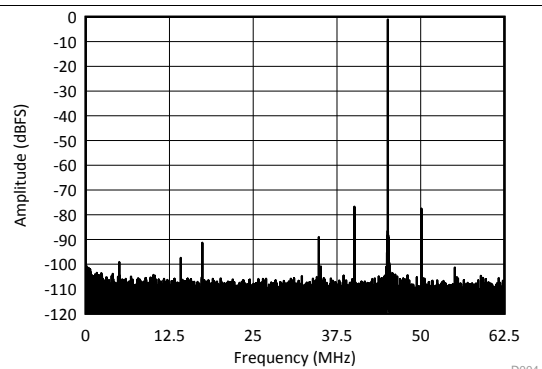
Figure 33. Power-Supply Rejection Ratio Spectrum
