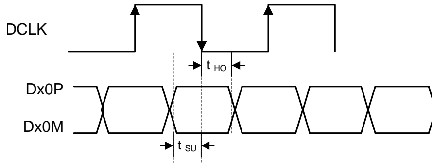
Figure 41. Setup and Hold Time
