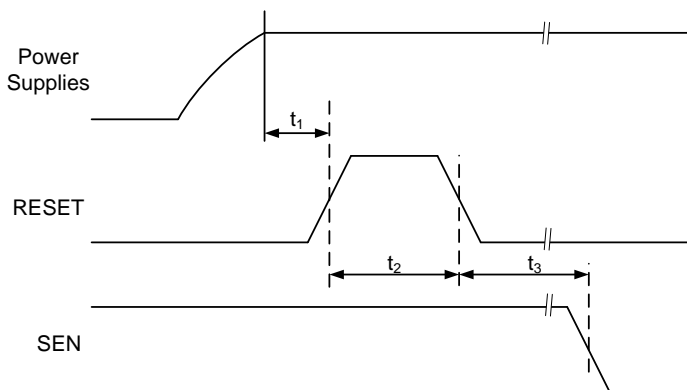
Figure 57. Initialization of Serial Registers after Power-Up
