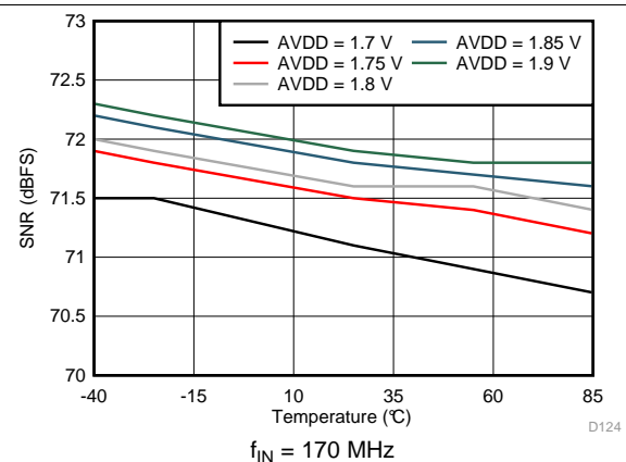
Figure 24. Signal-to-Noise Ratio vs AVDD Supply and Temperature
