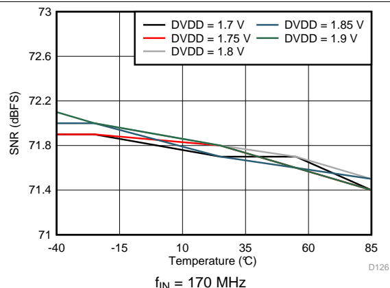
Figure 26. Signal-to-Noise Ratio vs DVDD Supply and Temperature
