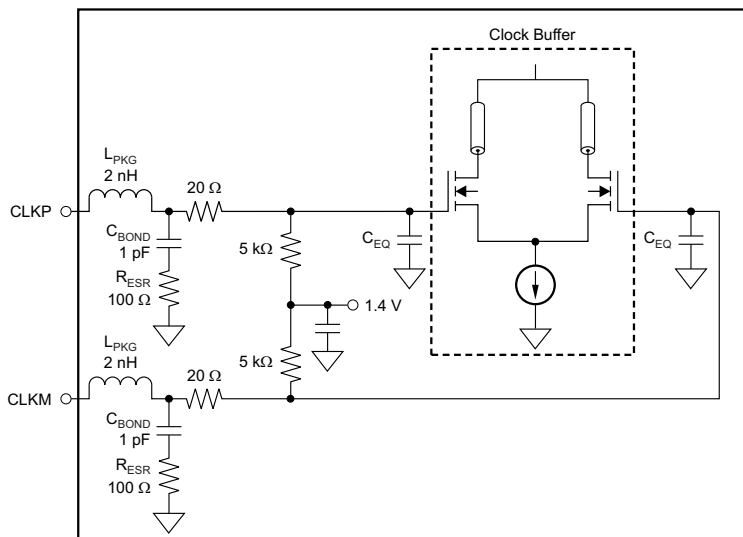
Figure 46. Internal Clock Buffer
