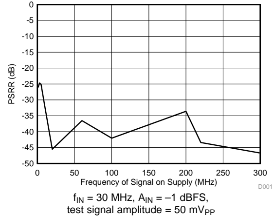
Figure 32. Power-Supply Rejection Ratio vs Test Signal Frequency
