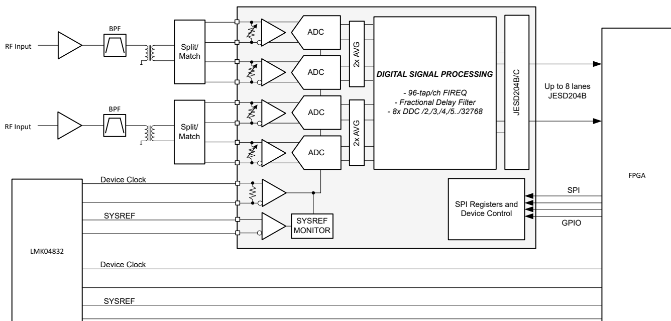
Figure 8-1. Wideband RF Sampling Receiver
