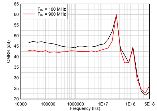
Figure 5-24. CMRR
