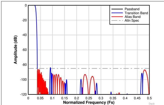
Figure 8-25. Decimation by 16 complex frequency response
