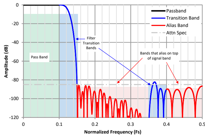
Figure 8-18. Interpretation of the Decimation Filter Plots
