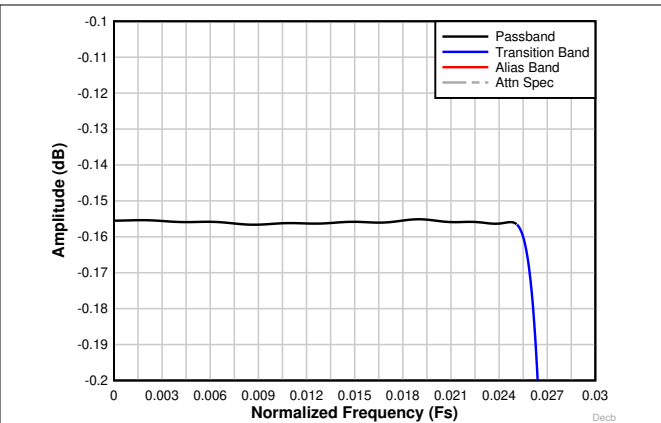
Figure 8-26. Decimation by 16 complex passband ripple response
