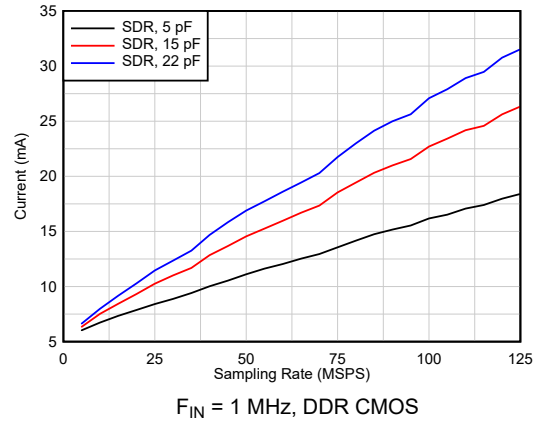
Figure 6-25. I_{IOVDD} Current vs Load Capacitance
