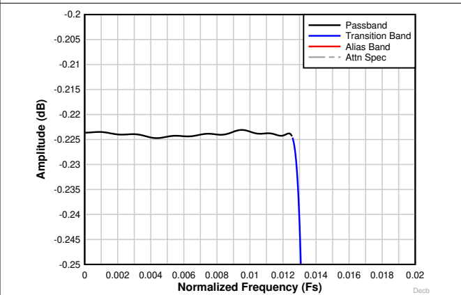
Figure 8-28. Decimation by 32 complex passband ripple response
