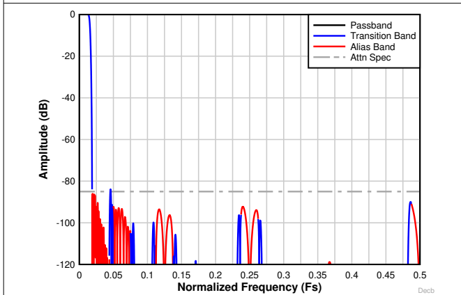
Figure 8-27. Decimation by 32 complex frequency response
