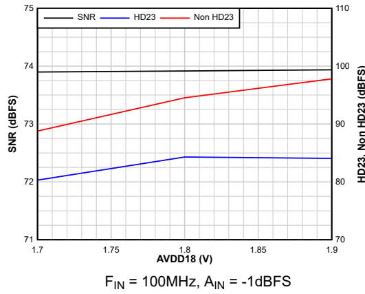
Figure 6-19. AC Performance vs AVDD18
