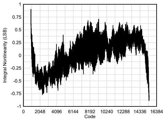
Figure 6-51. INL
