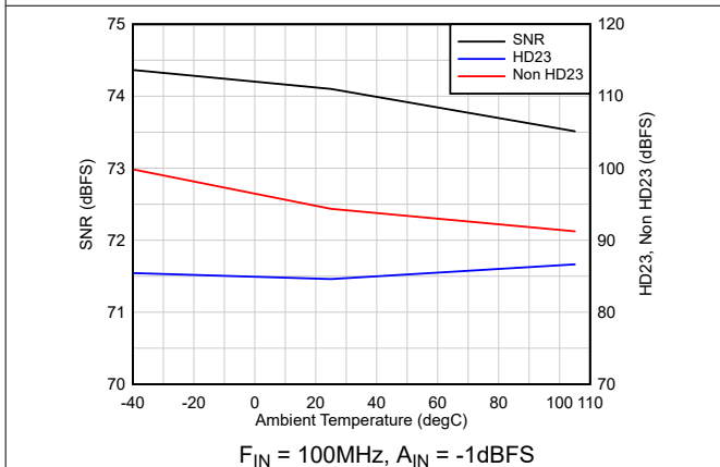
Figure 6-49. AC Performance vs Temperature
