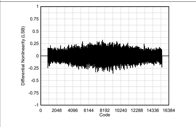
Figure 6-50. DNL
