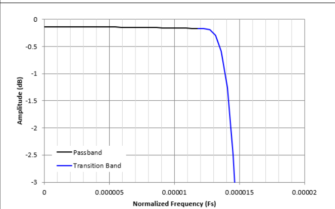
Figure 8-52. Decimation by 32768 Passband Ripple Response
