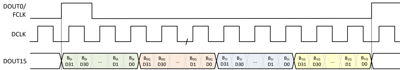
Figure 8-60. SLVDS frame assembly for example 4
