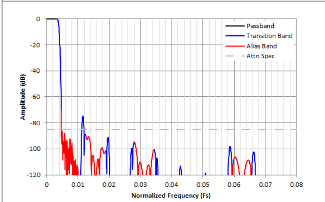
Figure 8-35. Complex Decimation by 128 Filter Response
