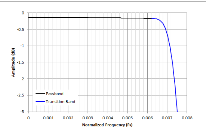
Figure 8-34. Complex Decimation by 64 Filter Ripple Response
