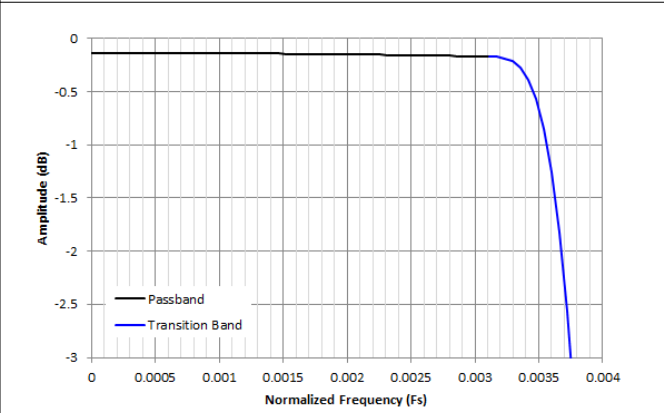
Figure 8-36. Decimation by 128 Passband Ripple Response
