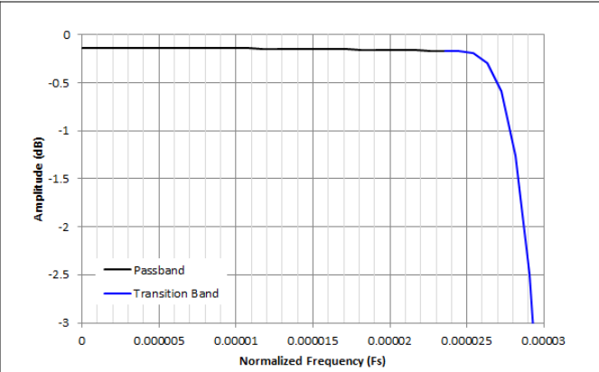
Figure 8-50. Decimation by 16384 Passband Ripple Response
