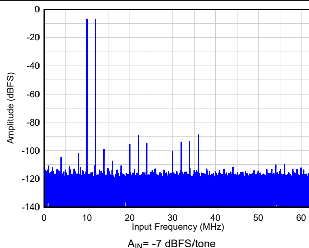
Figure 6-8. Two Tone FFT at F_{IN} = 10/12 MHz
