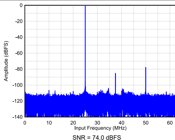
Figure 6-7. Single Tone FFT at F_{IN} = 100 MHz
