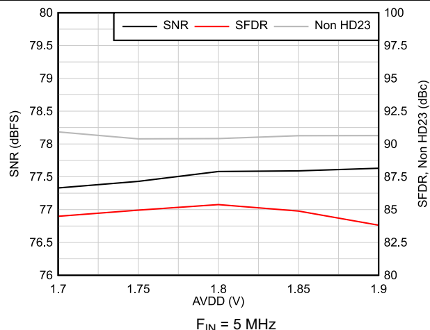
Figure 6-15. AC Performance vs AVDD
