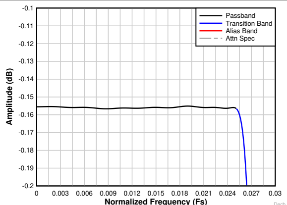
Figure 7-28. Decimation by 16 complex passband ripple response
