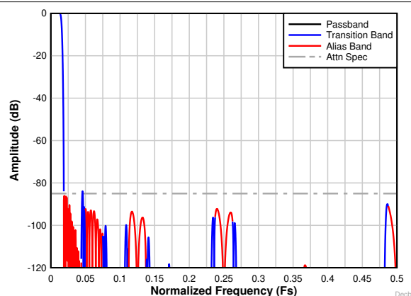
Figure 7-29. Decimation by 32 complex frequency response
