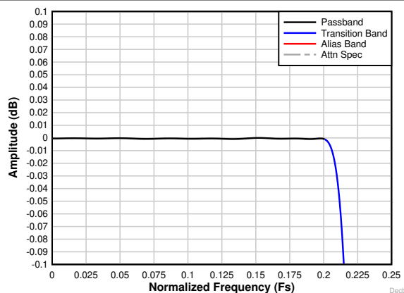
Figure 7-22. Decimation by 2 complex passband ripple response
