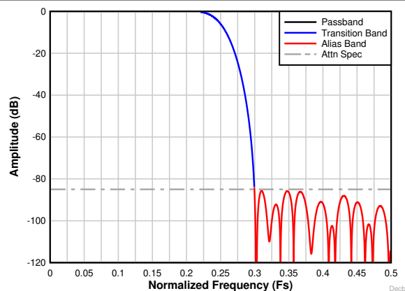
Figure 7-21. Decimation by 2 complex frequency response
