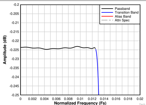
Figure 7-30. Decimation by 32 complex passband ripple response
