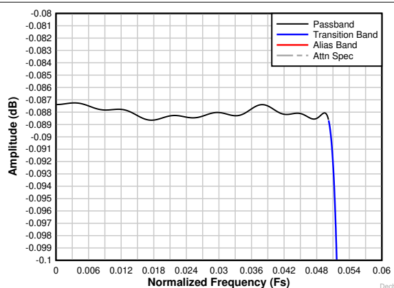
Figure 7-26. Decimation by 8 complex passband ripple response
