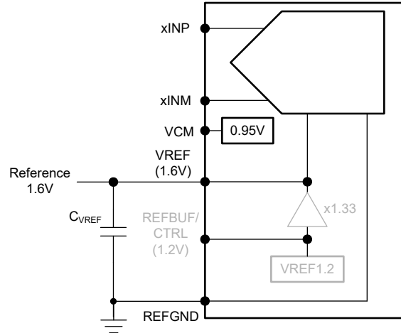
Figure 7-13. External 1.6V reference
