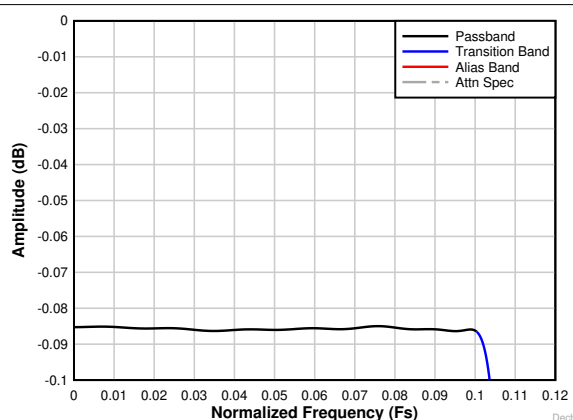
Figure 7-24. Decimation by 4 complex passband ripple response
