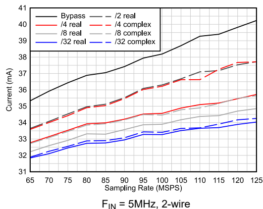
Figure 5-28. Power Consumption vs Decimation
