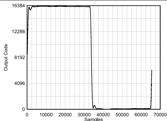
Figure 5-26. Pulse Response
