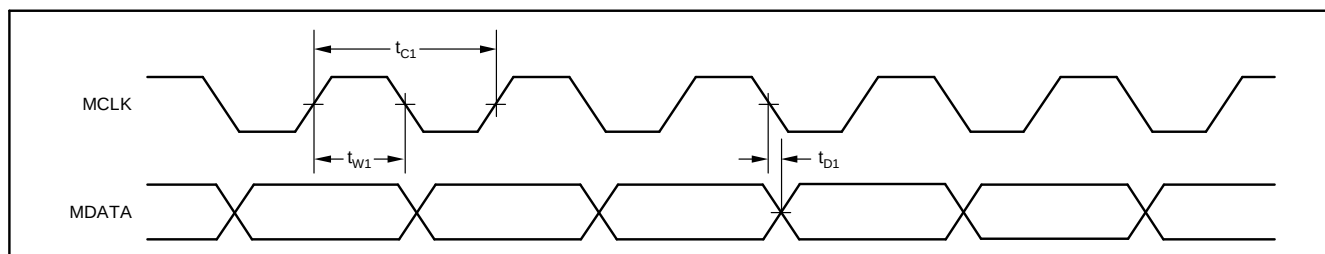
Figure 1. Mode 0 Operation
