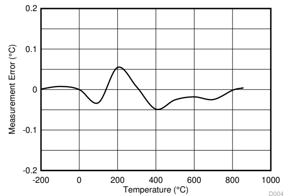
Figure 9-10. Temperature Measurement Error vs T_{RTD}
