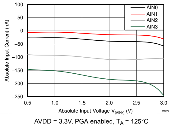
Figure 6-18. Absolute Input Current vs Absolute Input Voltage
