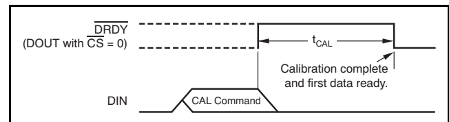
Figure 56. Calibration Timing
