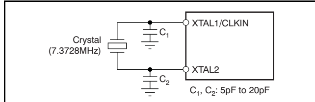
Figure 47. Crystal Connection
