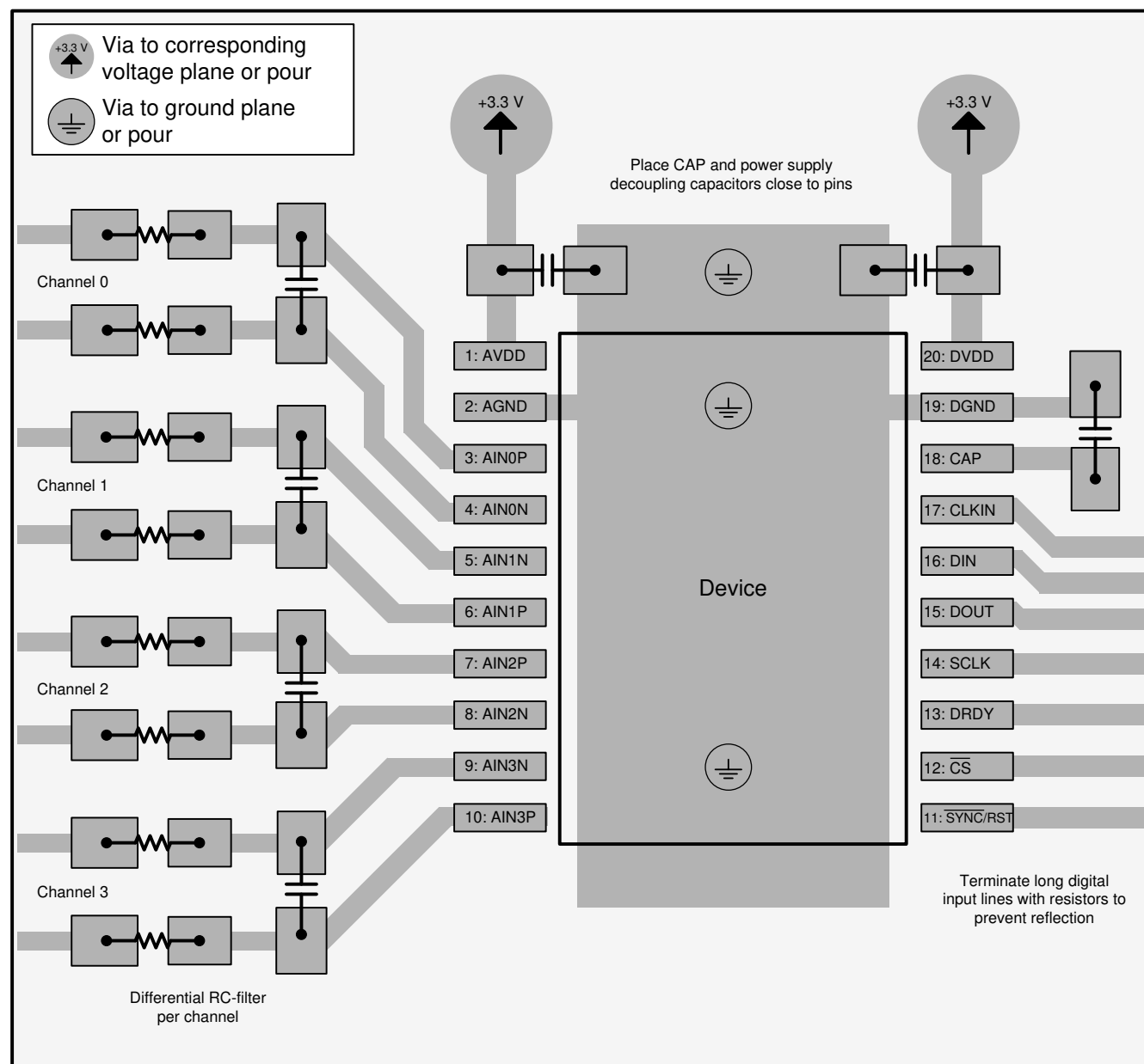
Figure 9-6. Layout Example
