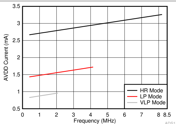
Figure 6-28. AVDD Current vs CLKIN Frequency
