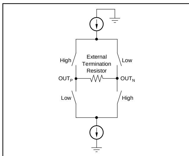
Figure 38. LVDS Buffer
