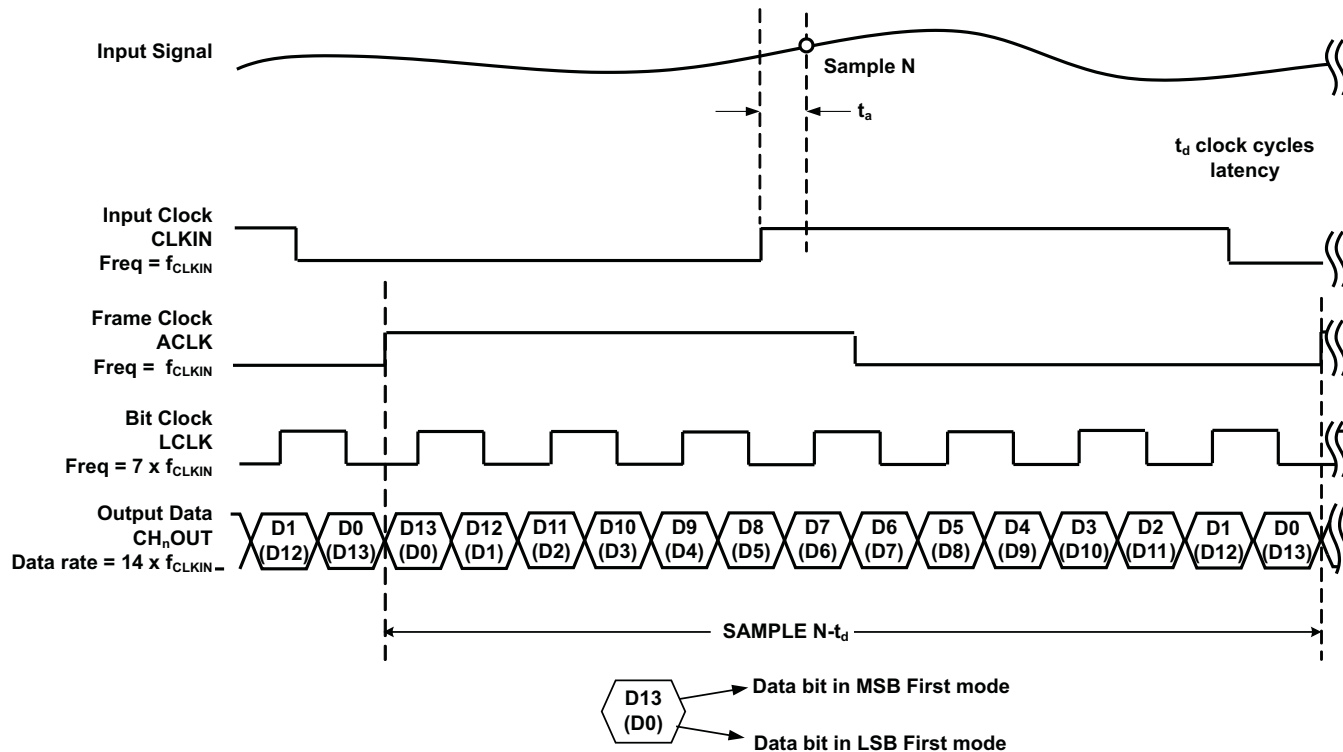
Figure 4. Enlarged 1-Wire LVDS Timing Diagram (14 bit)
