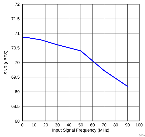
Figure 11. SIGNAL-TO-NOISE RATIO vs INPUT SIGNAL FREQUENCY
