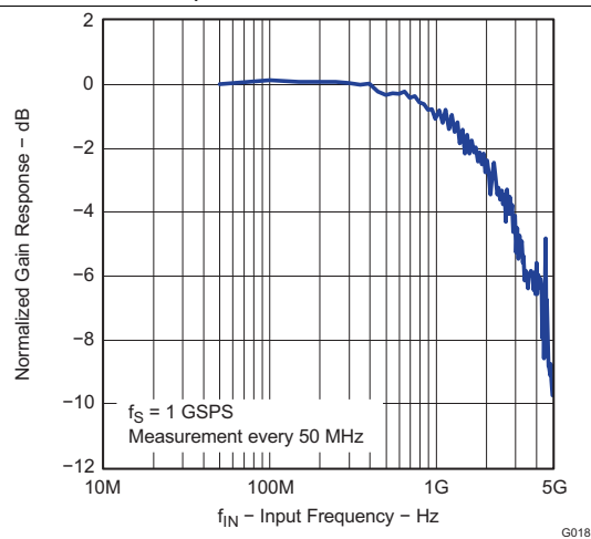
Figure 24. Normalized Gain Response vs Input Frequency
