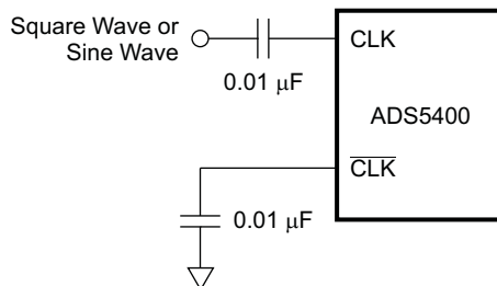
Figure 29. Single-Ended Clock
