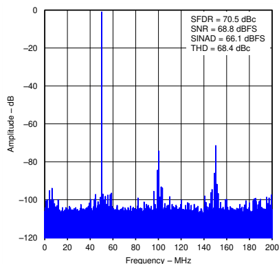
Figure 5-8. Spectral Performance FFT for 451MHz Input Signal
