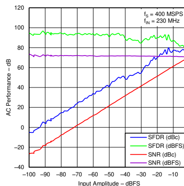
Figure 5-20. AC Performance vs Input Amplitude (230MHz Input Signal)
