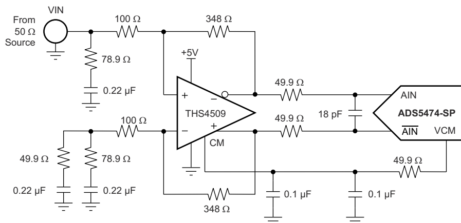
Figure 6-4. Using the THS4509 or THS4520 With the ADS5474
