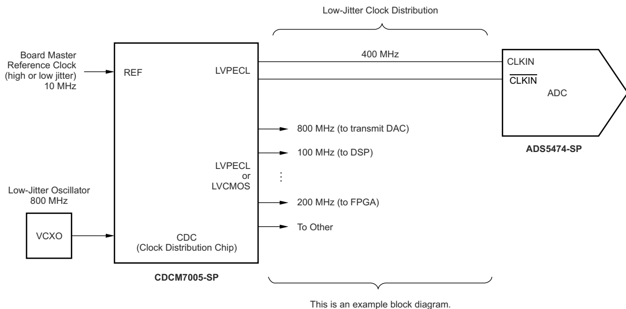
Figure 6-8. Best Jitter Clock Circuit
