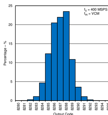
Figure 5-18. Noise Histogram With Inputs Shorted
