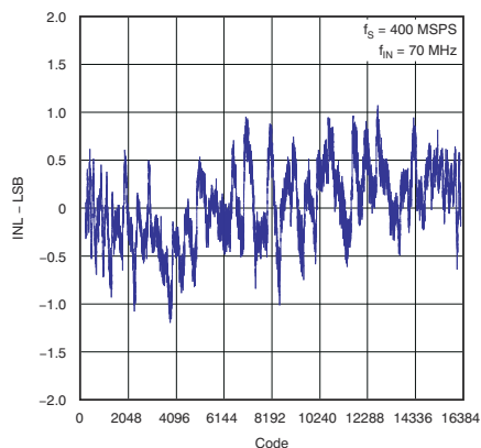
Figure 5-17. Integral Nonlinearity
