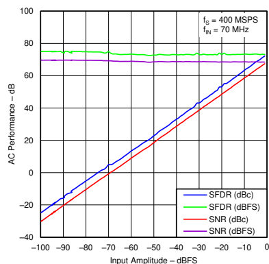
Figure 5-19. AC Performance vs Input Amplitude (70MHz Input Signal)
