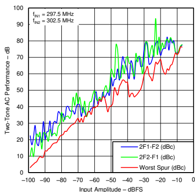
Figure 5-21. Two-Tone Performance vs Input Amplitude ( F1 = 297.5\text{MHz} and F2 = 302.5\text{MHz} )
