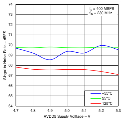
Figure 5-23. SNR vs AVDD5 Over Temperature
