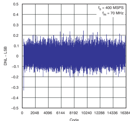
Figure 5-16. Differential Nonlinearity
