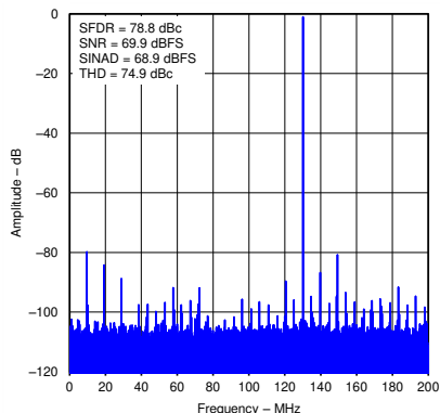
Figure 5-5. Spectral Performance FFT for 130MHz Input Signal
