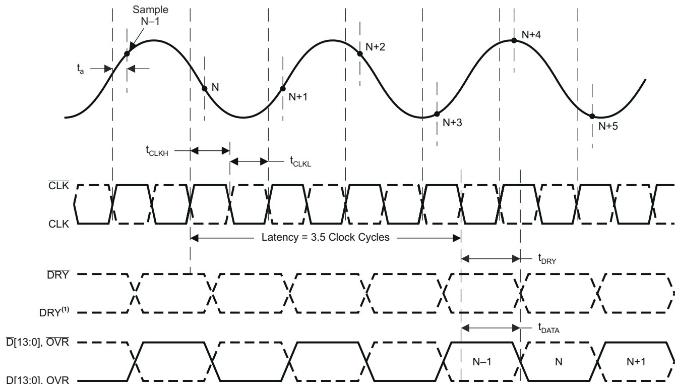
Figure 5-2. Timing Diagram
