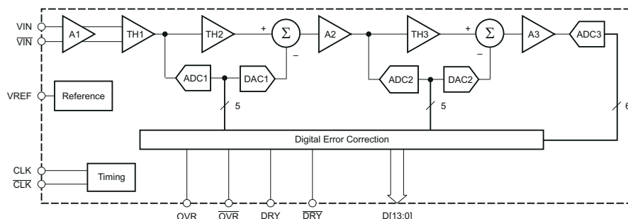
Simplified Schematic
