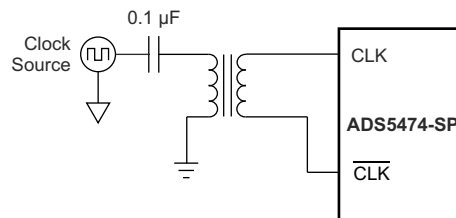
Figure 6-7. Differential Clock
