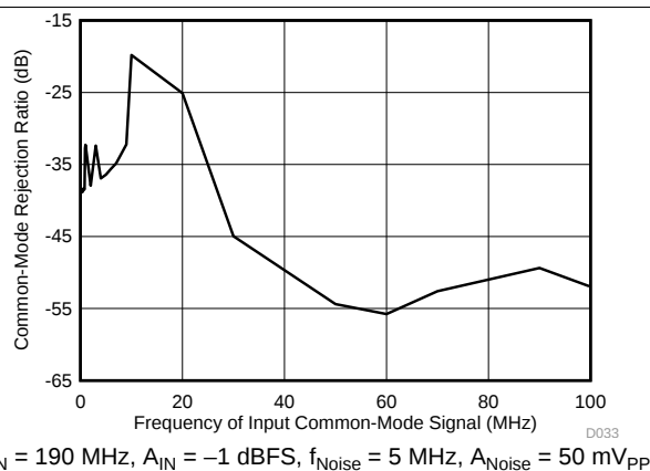
Figure 34. CMRR vs Common-Mode Noise Frequency
