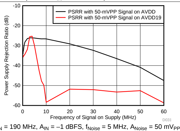
Figure 32. PSRR vs Power-Supply Noise Frequency
