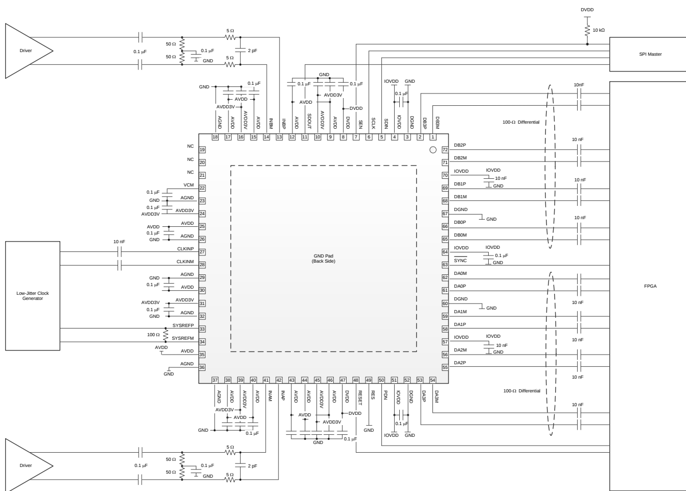
Figure 131. AC-Coupled Receiver
