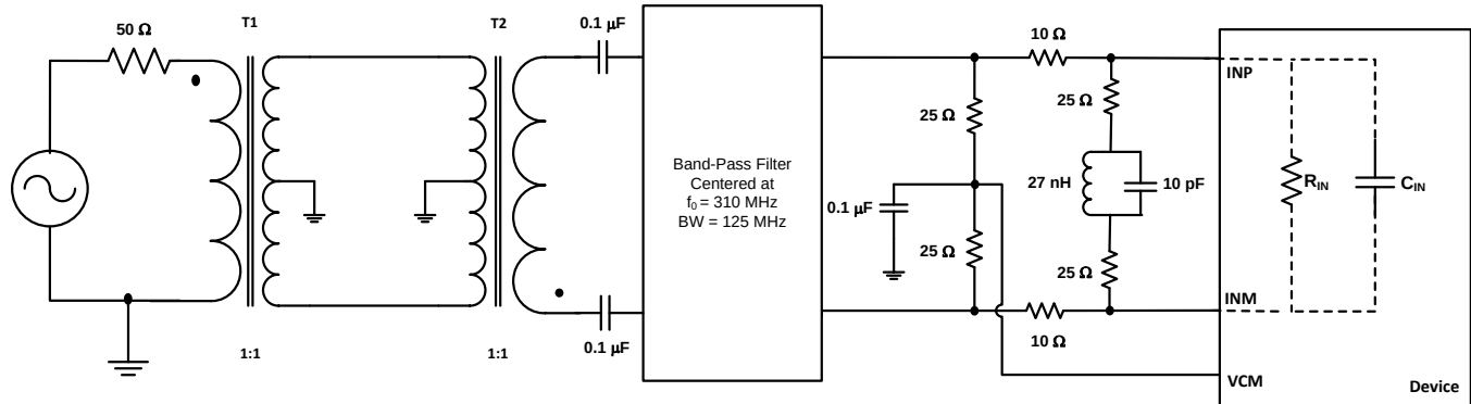
Figure 47. Driving Circuit for a 50- \Omega Source Impedance and Input Frequencies in the Third Nyquist Zone
