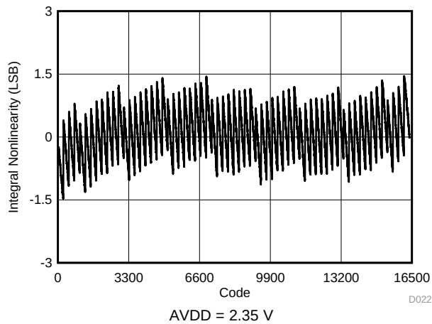
Figure 23. Typical INL
