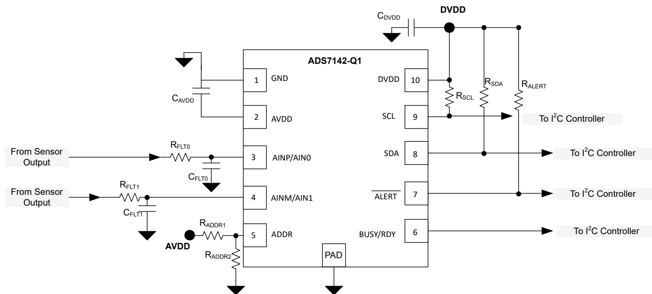
Figure 8-10. Example Schematic
