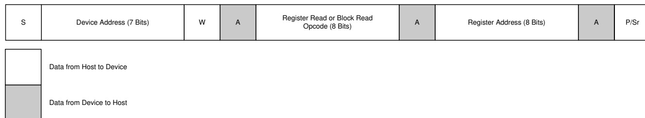
Figure 7-26. Setting Register Address for Reading Registers
