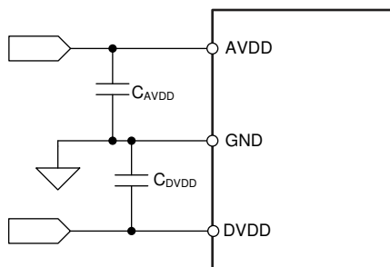
Figure 8-9. Power-Supply Decoupling
