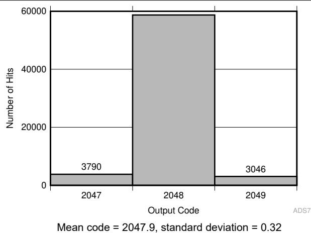
Figure 6-12. Typical DC Code Spread in Manual Mode
