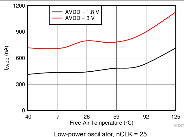
Figure 6-35. I_{AVDD} in High-Precision Mode vs Temperature
