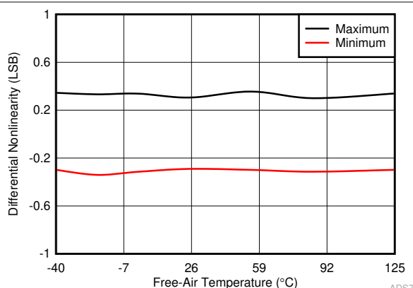
Figure 6-21. DNL in Manual Mode vs Temperature
