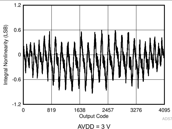
Figure 6-19. Typical INL in Manual Mode
