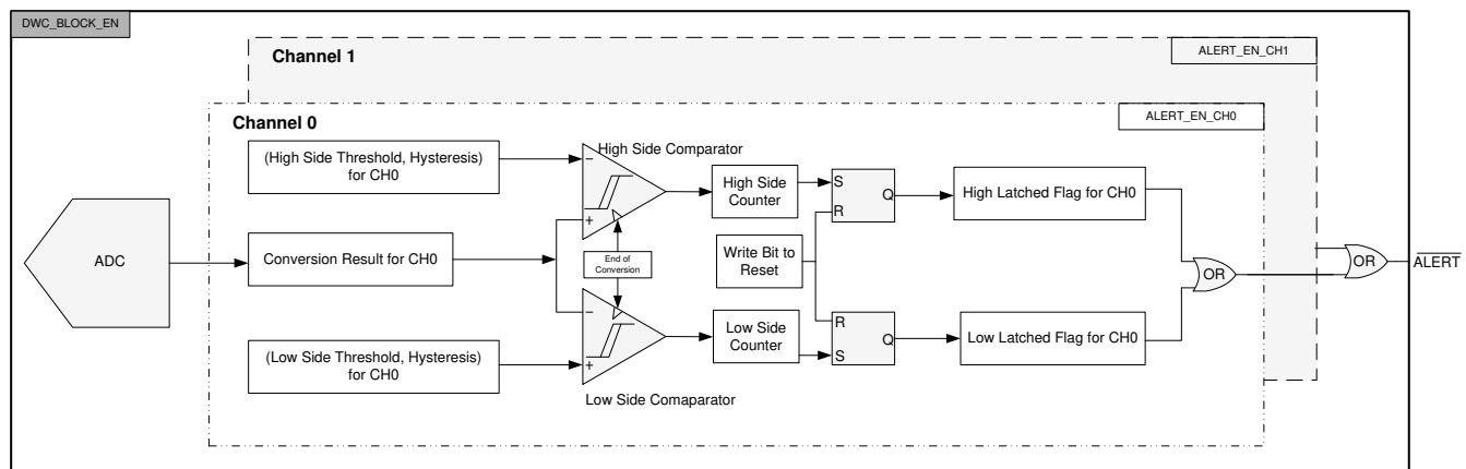
Figure 7-9. Digital Comparator Block Diagram
