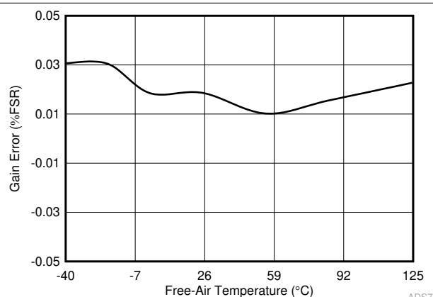
Figure 6-15. Gain Error in Manual Mode vs Free-Air Temperature
