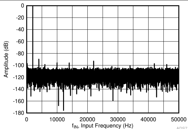
Figure 6-6. Typical FFT in Manual Mode
