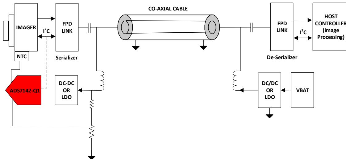
Figure 8-8. Voltage and Temperature Sensing in Remote Camera Modules Using the ADS7142-Q1
