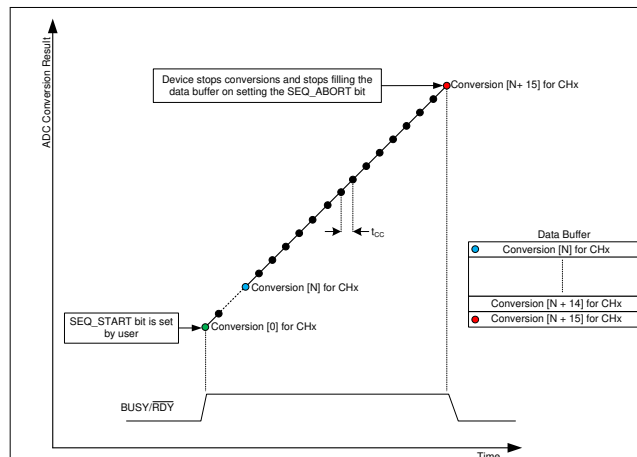
Figure 7-21. Stop Burst With a Single-Channel Configuration
