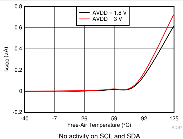
Figure 6-28. Static I_{AVDD} in Manual Mode vs Temperature
