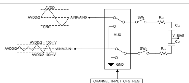
Figure 7-4. Single-Channel, Pseudo-Differential Configuration
