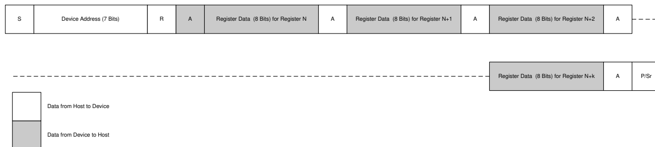
Figure 7-28. Reading a Continuous Block of Registers
