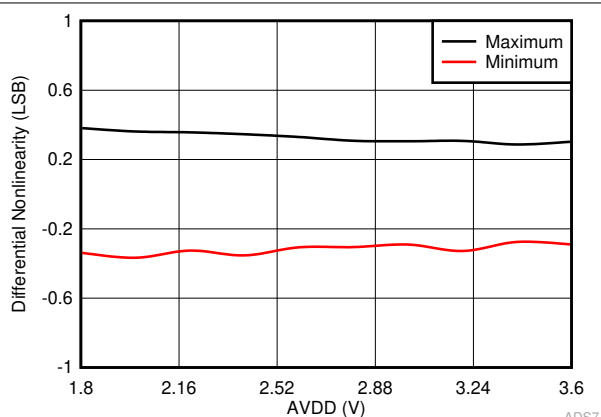
Figure 6-22. DNL in Manual Mode vs AVDD
