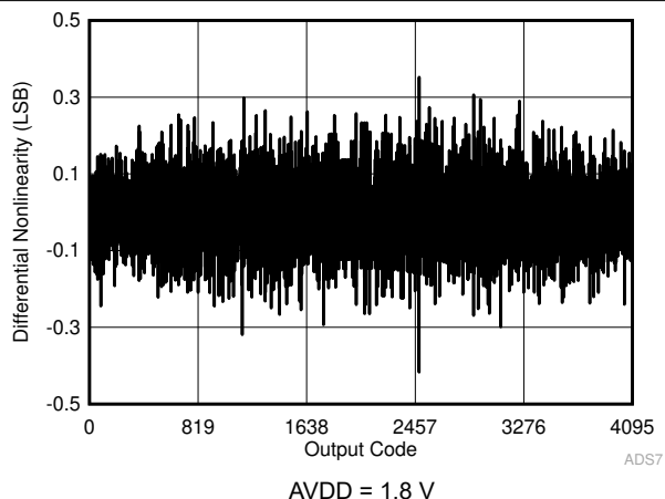
Figure 6-18. Typical DNL in Manual Mode
