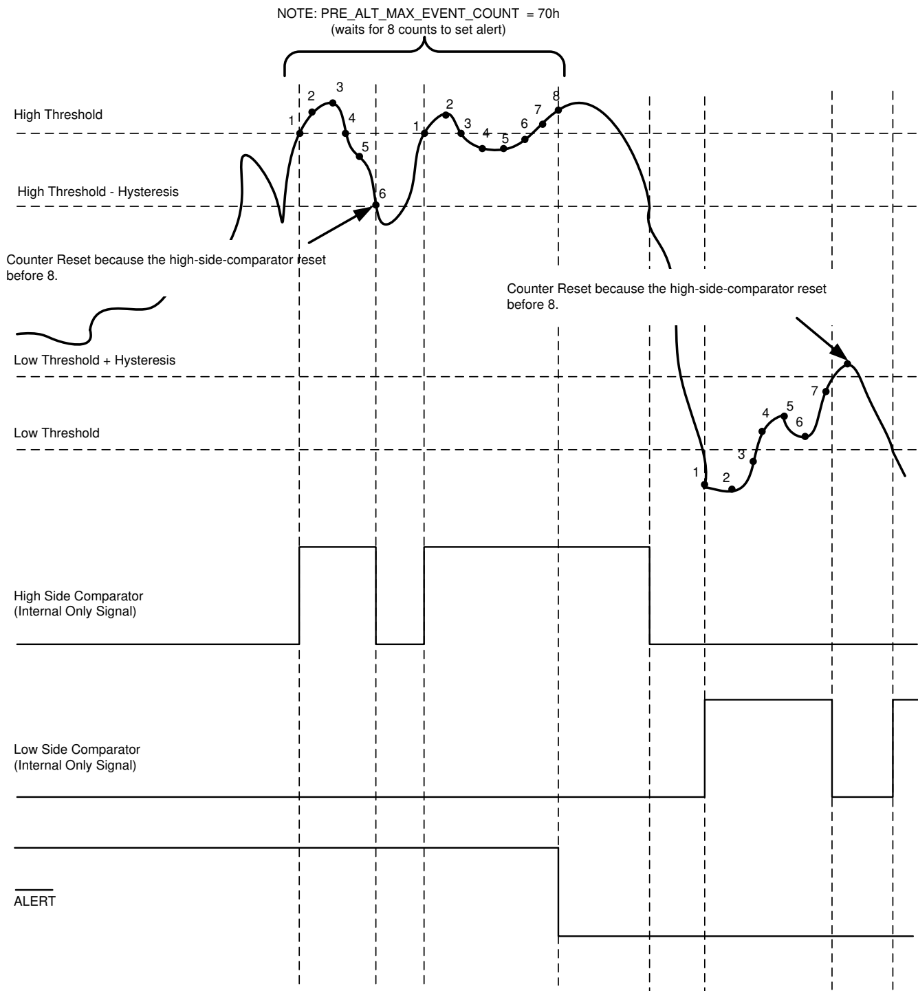
Figure 7-10. Thresholds, Hysteresis, and Event Counter for the Digital Window Comparator
