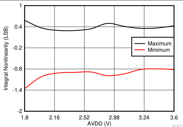
Figure 6-24. INL in Manual Mode vs AVDD
