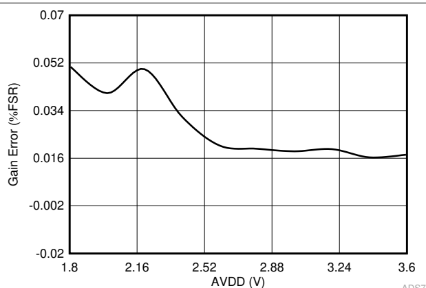
Figure 6-16. Gain Error in Manual Mode vs AVDD
