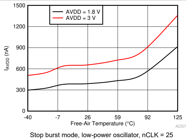
Figure 6-31. I_{AVDD} in Autonomous Modes vs Temperature
