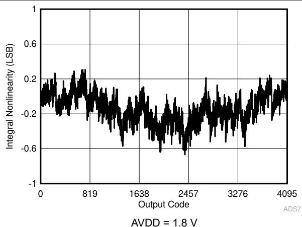
Figure 6-20. Typical INL in Manual Mode
