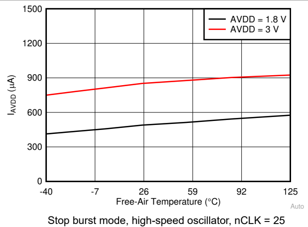
Figure 6-32. I_{AVDD} in Autonomous Modes vs Temperature
