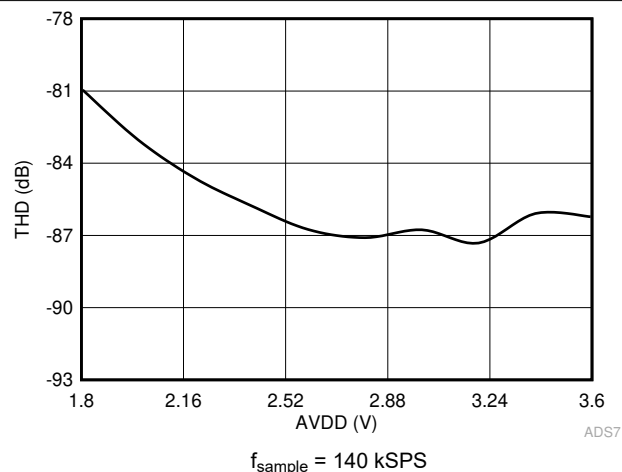
Figure 6-11. THD in Manual Mode vs AVDD
