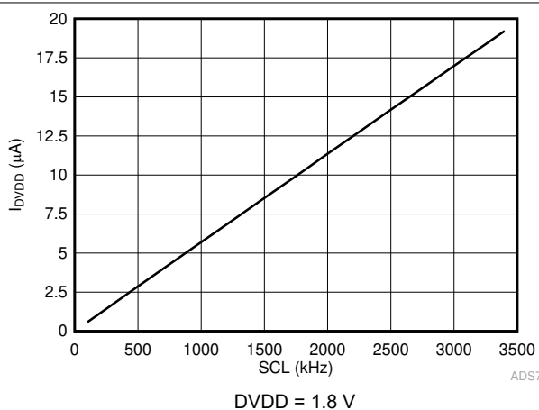
Figure 6-27. I_{DVDD} in Manual Mode vs SCL
