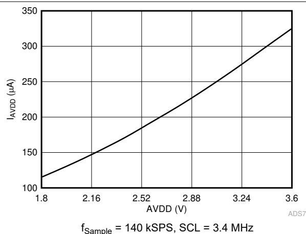
Figure 6-25. I_{AVDD} in Manual Mode vs AVDD
