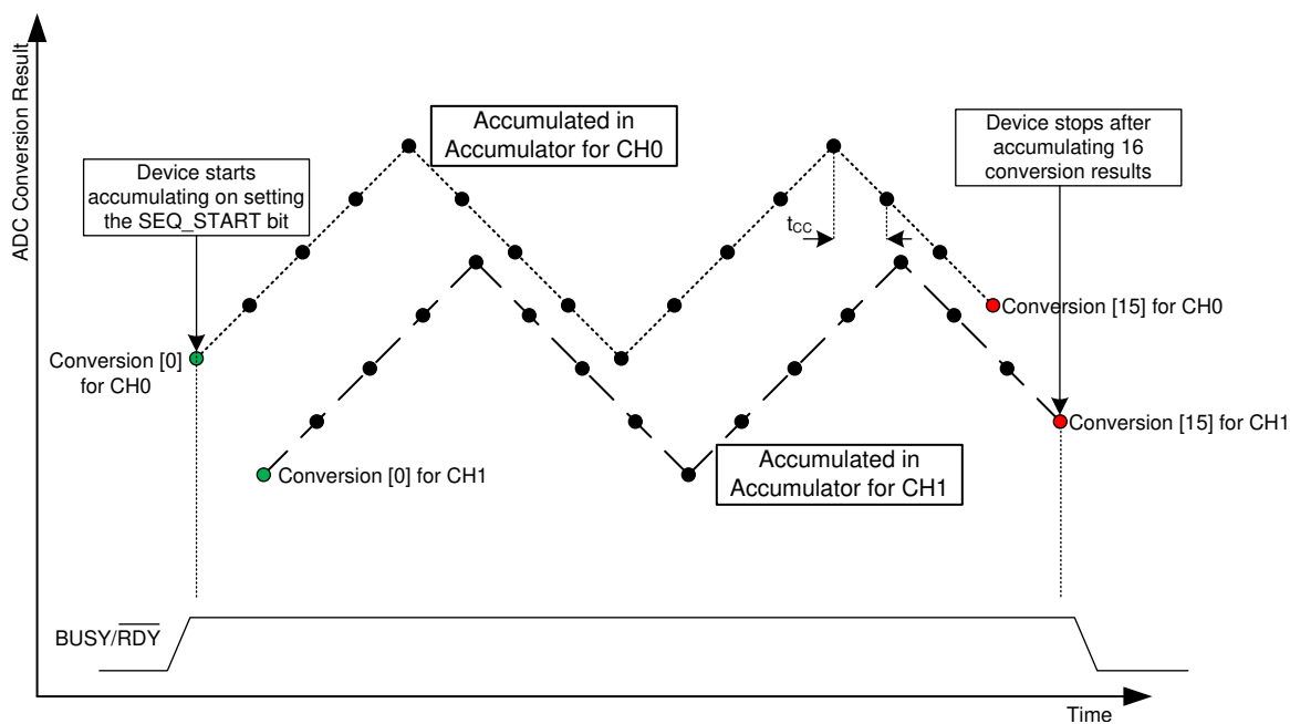
Figure 7-25. High-Precision Mode With Dual-Channel Configurations
