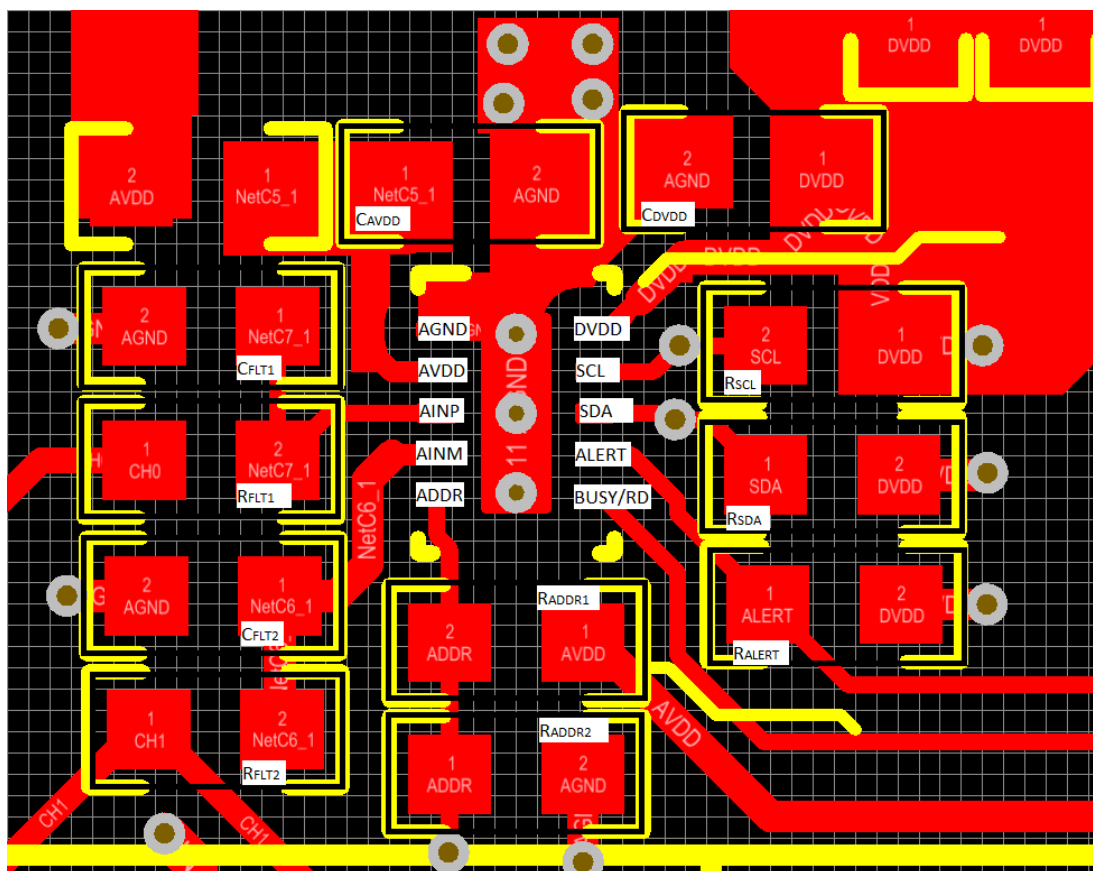
Figure 8-11. Example Layout
