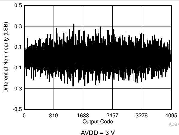
Figure 6-17. Typical DNL in Manual Mode
