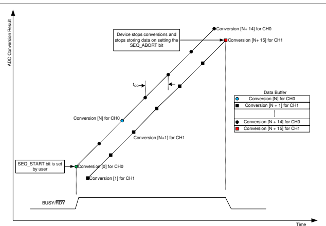
Figure 7-22. Stop Burst With a Dual-Channel Configuration
