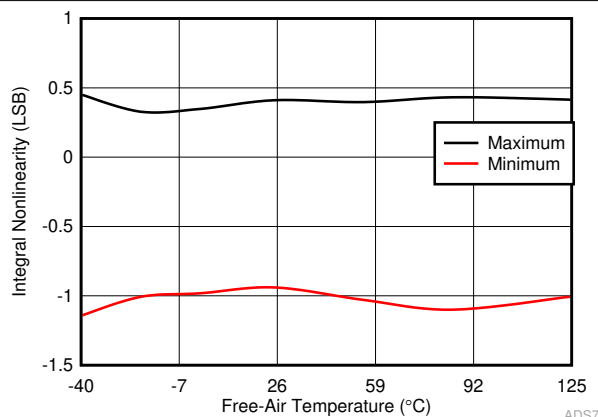
Figure 6-23. INL in Manual Mode vs Temperature
