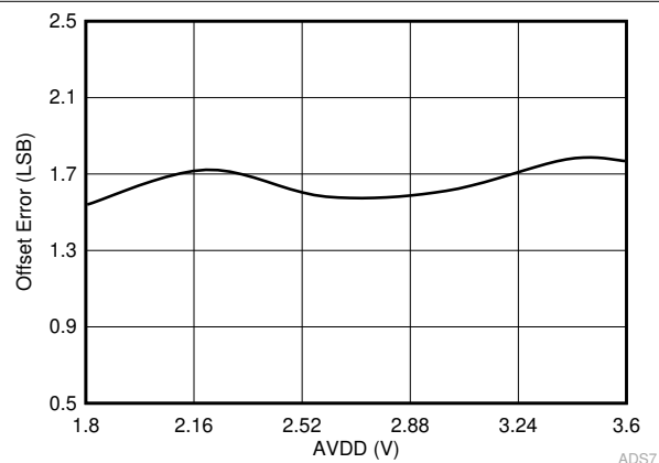
Figure 6-14. Offset Error in Manual Mode vs AVDD
