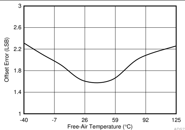
Figure 6-13. Offset Error in Manual Mode vs Temperature
