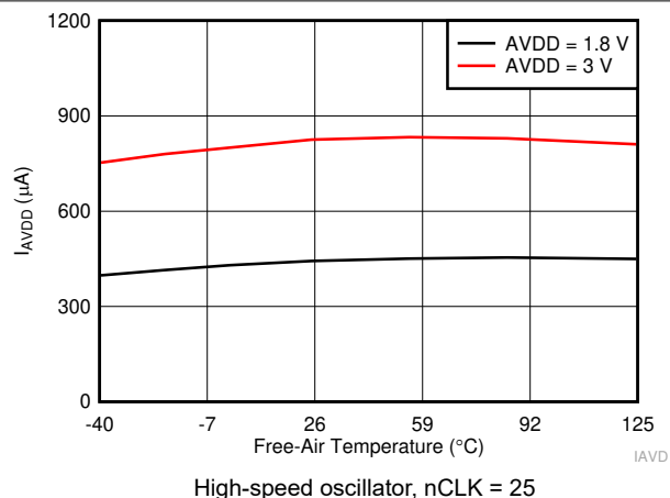
Figure 6-36. I_{AVDD} in High-Precision Mode vs Temperature
