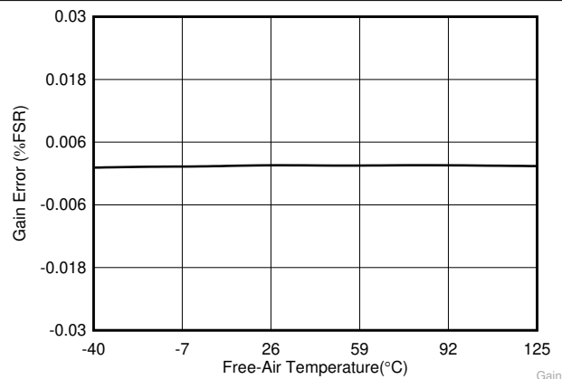
Figure 6-34. Gain Error in High-Precision Mode vs Temperature
