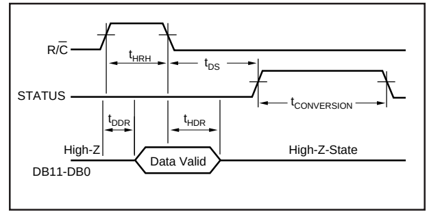
FIGURE 4. R/\bar{C} Pulse High — Outputs Enabled Only While R/\bar{C} Is High.
