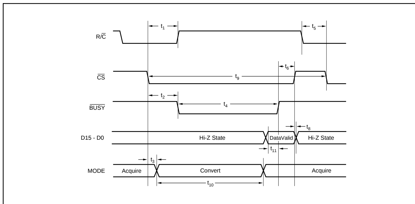
FIGURE 2. ADS7815 Timing.
