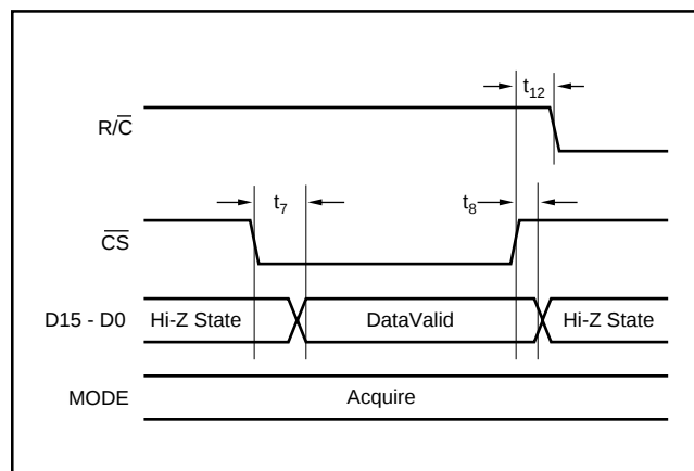
FIGURE 3. Bus Timing.
