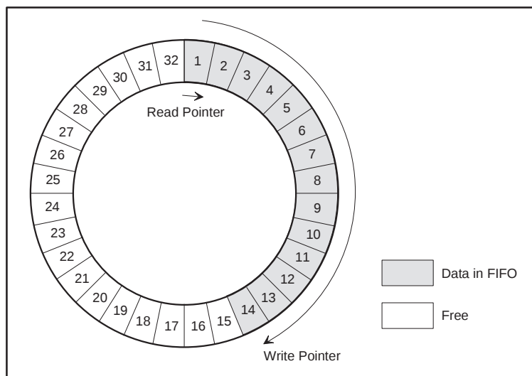
Figure 1–20. FIFO Structure
