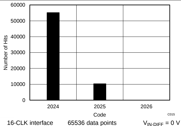
Figure 68. DC Histogram
