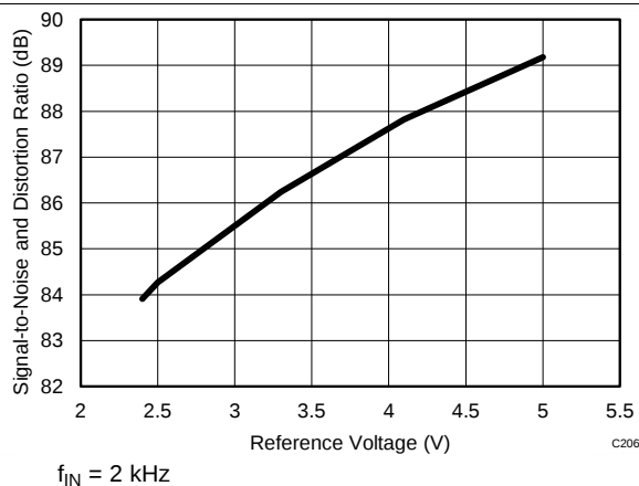
Figure 7. SINAD vs Reference Voltage
