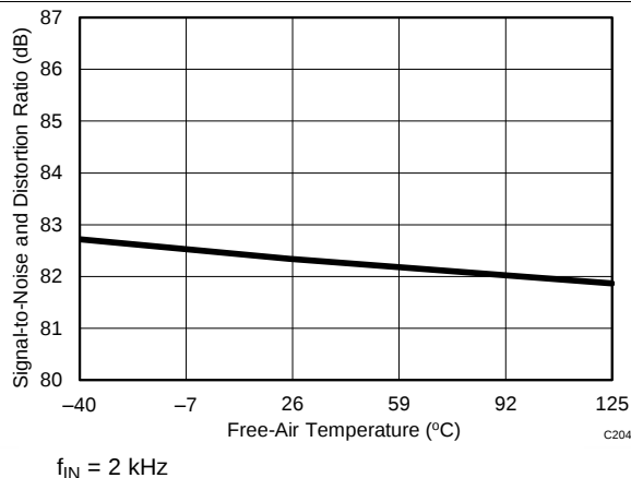
Figure 5. SINAD vs Temperature
