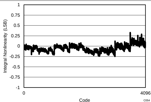
Figure 73. Typical INL
