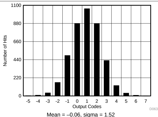
Figure 73. DC Histogram for OSR4
