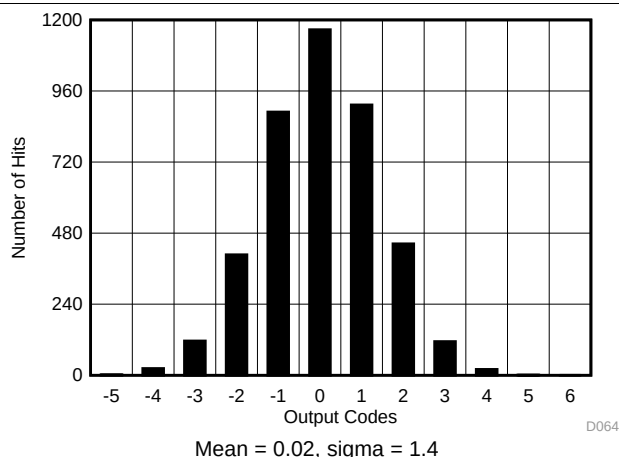
Figure 74. DC Histogram for OSR8
