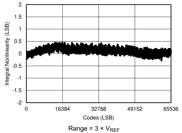
Figure 6-15. Typical INL for All Codes
