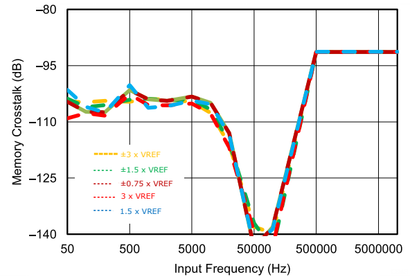
Figure 6-41. Memory Crosstalk vs Frequency for Overrange Inputs
