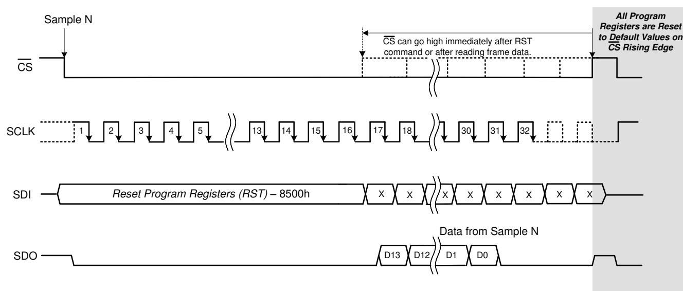
Figure 7-40. Reset Program Registers (RST) Timing Diagram
