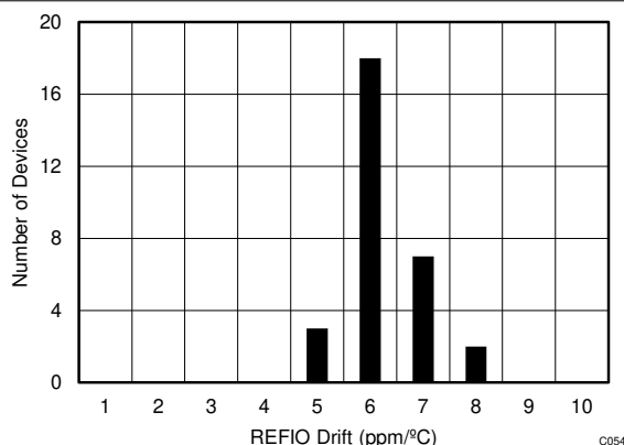
Figure 7-11. Internal Reference Temperature Drift Histogram
