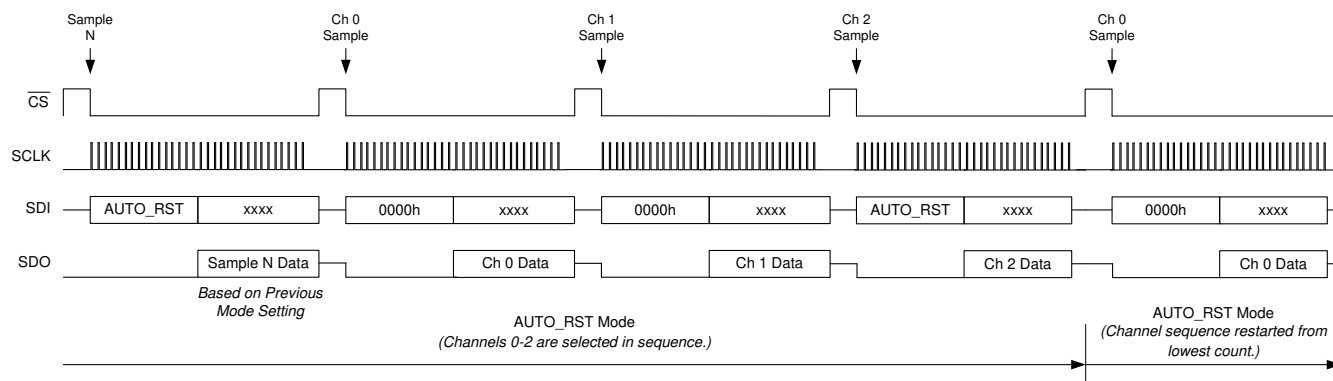
Figure 7-35. Device Operation Example in AUTO_RST Mode
