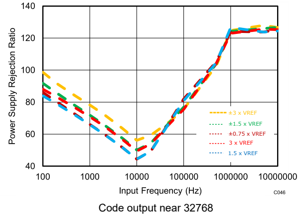
Figure 9-3. PSRR With a Decoupling Capacitor
