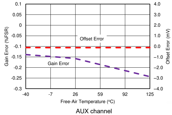
Figure 7-16. Offset and Gain vs Temperature (AUX Channel)
