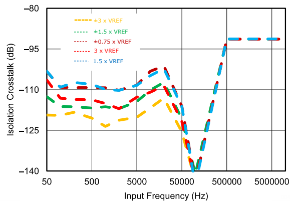
Figure 6-42. Isolation Crosstalk vs Frequency for Overrange Inputs
