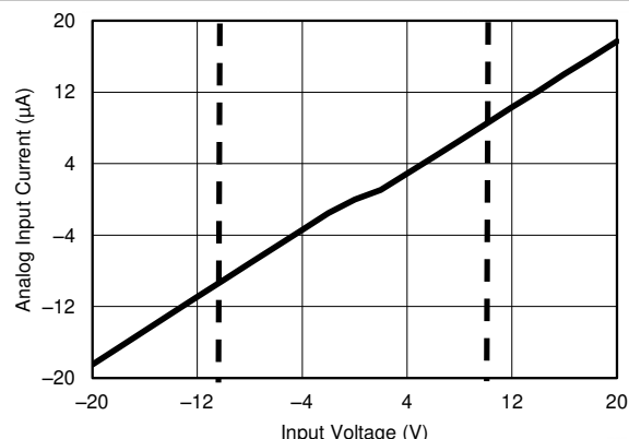
Figure 7-4. I-V Curve for an Input OVP Circuit (AVDD = Floating)
