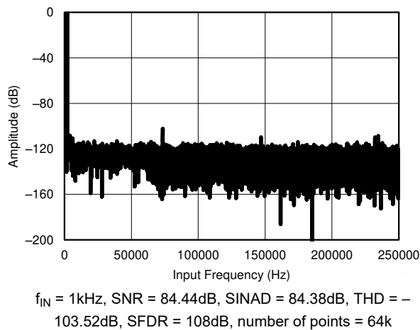
Figure 7-17. Typical FFT Plot (AUX Channel)
