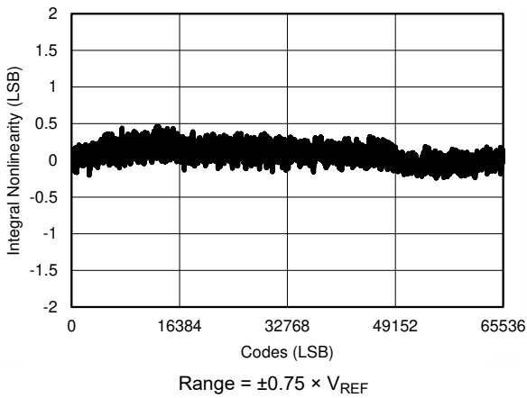
Figure 6-14. Typical INL for All Codes
