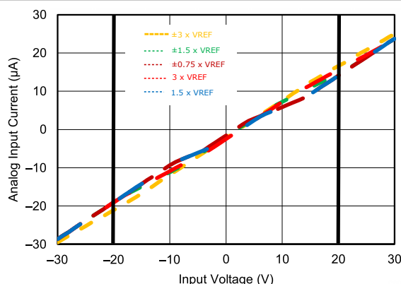
Figure 7-3. I-V Curve for an Input OVP Circuit (AVDD = 5V)
