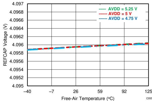
Figure 7-13. Variation of the Reference Buffer Output (REFCAP) vs Supply and Temperature
