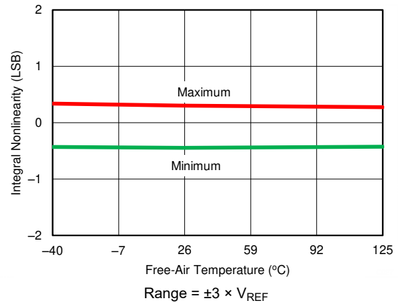
Figure 6-17. INL vs Temperature ( \pm 3 \times V_{REF} )
