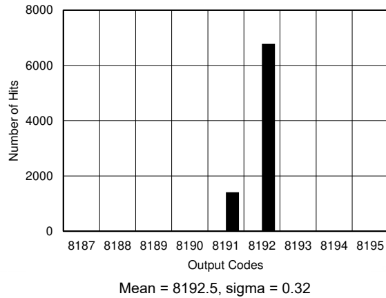
Figure 7-15. DC Histogram for Mid-Scale Input (AUX Channel)
