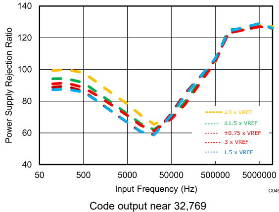
Figure 9-2. PSRR Without a Decoupling Capacitor
