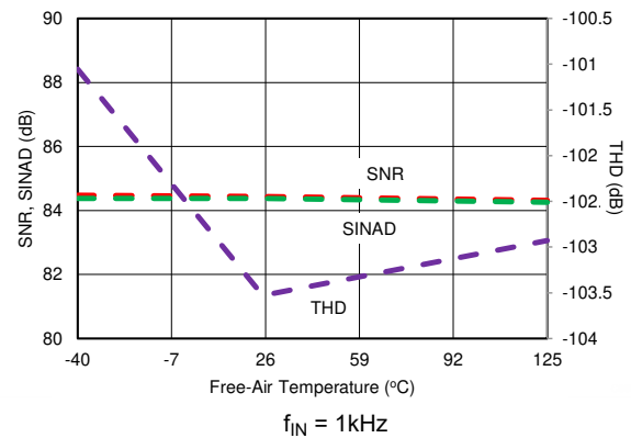
Figure 7-18. SNR, SINAD, and THD vs Temperature (AUX Channel)
