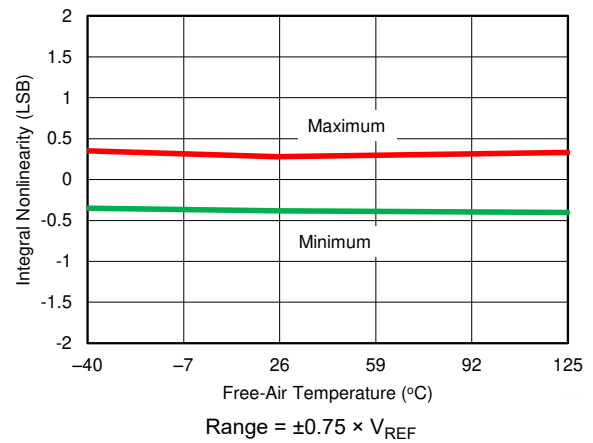
Figure 6-19. INL vs Temperature ( \pm 0.75 \times V_{REF} )
