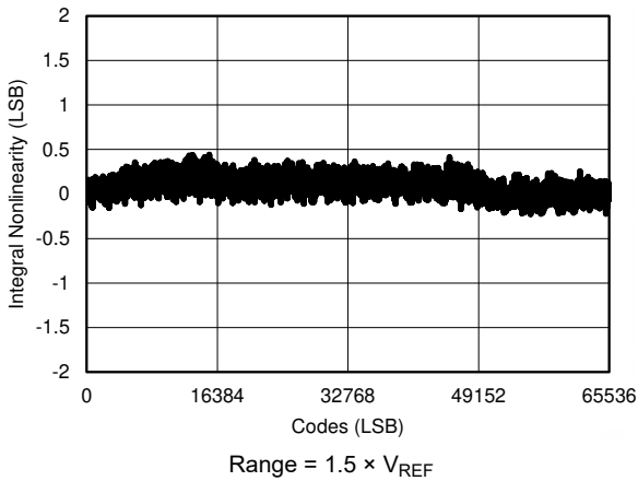
Figure 6-16. Typical INL for All Codes
