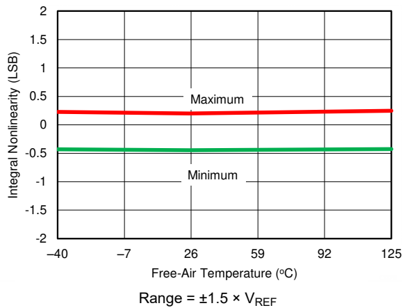
Figure 6-18. INL vs Temperature ( \pm 1.5 \times V_{REF} )
