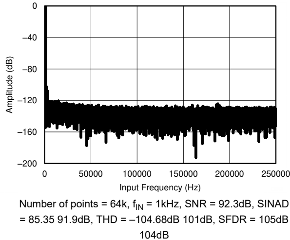
Figure 6-28. Typical FFT Plot ( \pm 3 \times V_{REF} )
