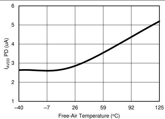
Figure 6-45. AVDD Current vs Temperature (Power Down)
