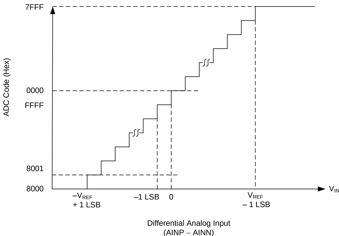
Figure 49. Transfer Characteristics
