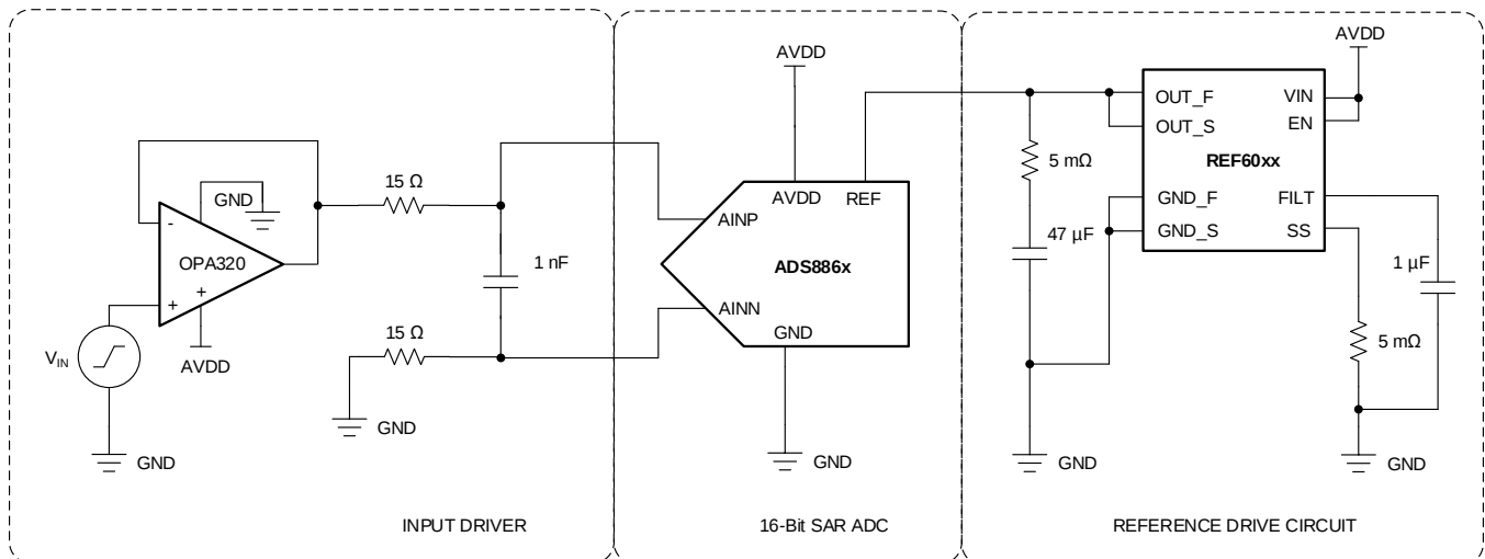
Figure 63. DAQ Circuit for a 1.5- \mu s, Full-Scale Step Response
