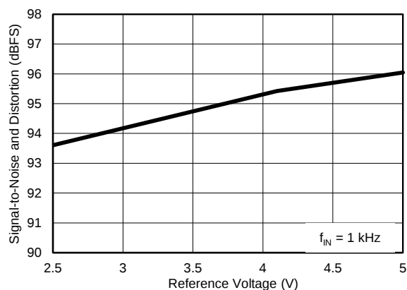
Figure 19. SINAD vs REFERENCE VOLTAGE
