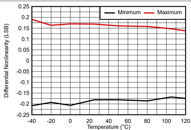
Figure 6-24. DNL vs Temperature
