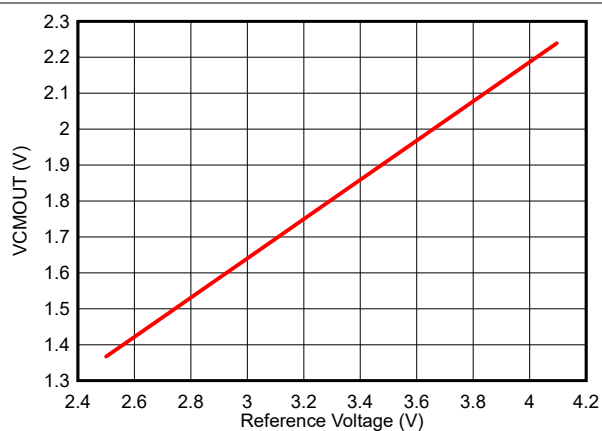
Figure 6-46. VCMOUT Voltage vs Reference Voltage
