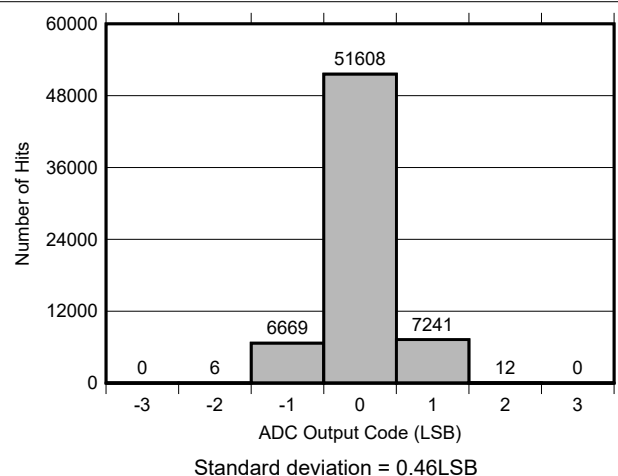
Figure 6-22. DC Input Histogram
