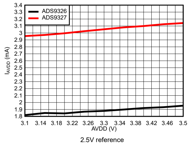
Figure 6-38. AVDD Current vs AVDD Voltage with Low AVDD
