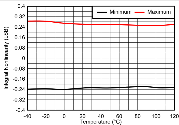
Figure 6-23. INL vs Temperature
