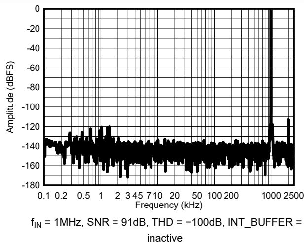
Figure 6-15. Typical FFT for f_{IN} = 1\text{MHz}
