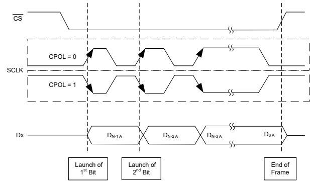
Figure 7-20. SPI-01 and SPI-11 Protocols
