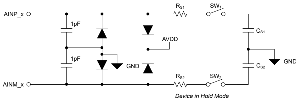
Figure 7-1. Analog Inputs
