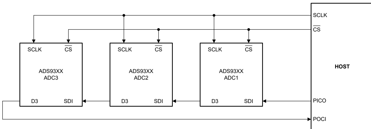
Figure 7-24. Daisy-Chain Connections
