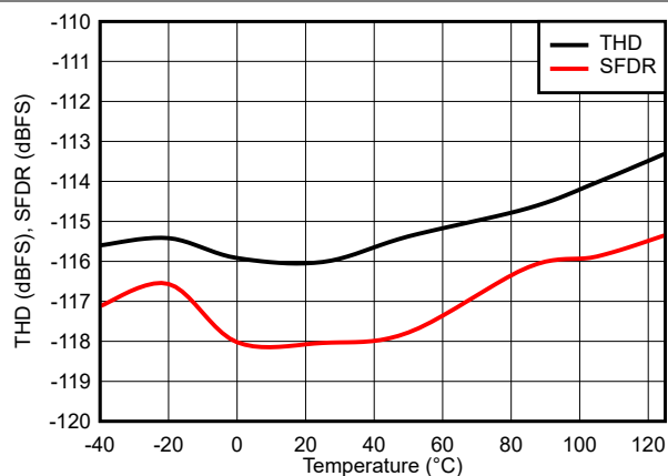
Figure 6-30. THD and SFDR vs Temperature
