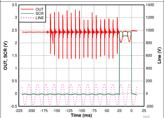
Figure 20. Device Trip to 2\text{-}\Omega N-G Fault. No Load Or Fault Currents.
