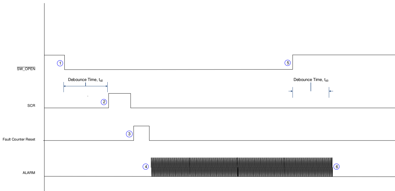
Figure 13. ALARM With \overline{\text{SW\_OPEN}} Transition to Low. No Self-Test Failure.
