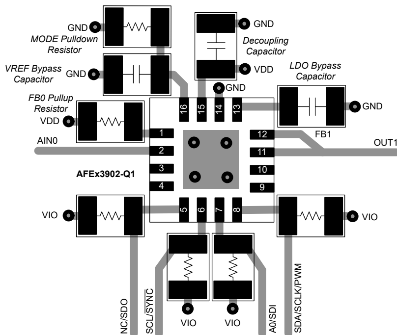
Figure 8-4. Layout Example
