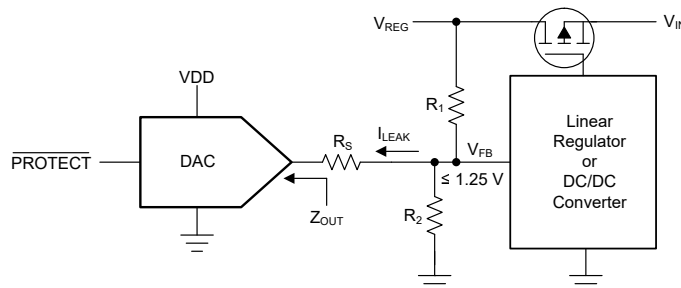
Figure 6-13. High-Impedance (Hi-Z) Output and \overline{\text{PROTECT}} Input
