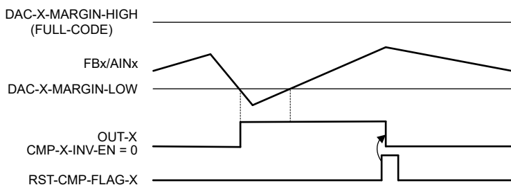
Figure 6-10. Latching Comparator With Active High Output
